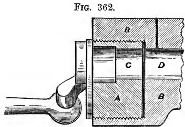
Clay's breech-loader.
