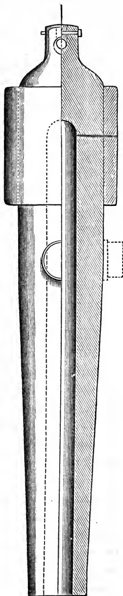
Parrott 6.4 inch "100-pounder" rifle, \frac{7}{8} in. to 1 ft.
