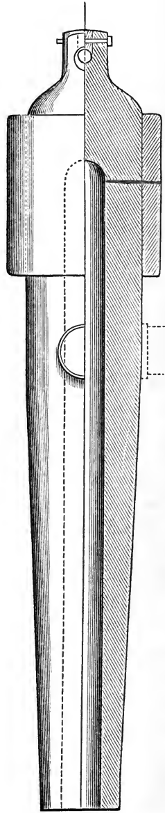
FIG. 45. Parrott 8-inch rifle. \frac{7}{8} in. to 1 ft.
