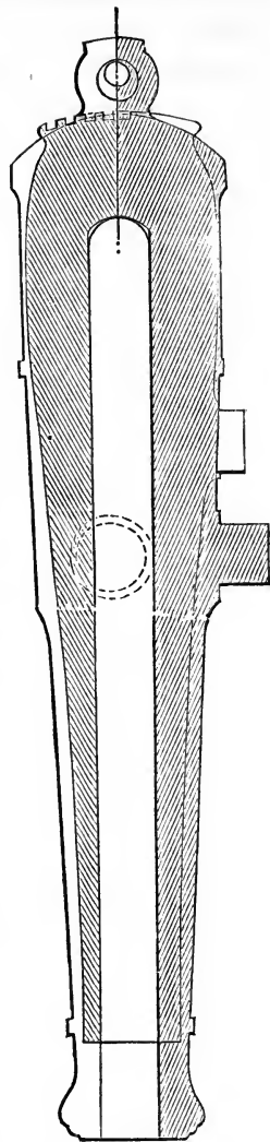
Section of British 8-in. (68-pdr.) laid over section of U. S. 8-in. Columbiad. Scale, \frac{1}{16} in. to 1 ft.
