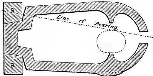
Haddan's projectile for wood sabot.
