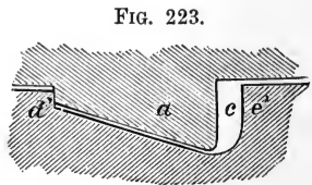
Scott's groove and rib.
