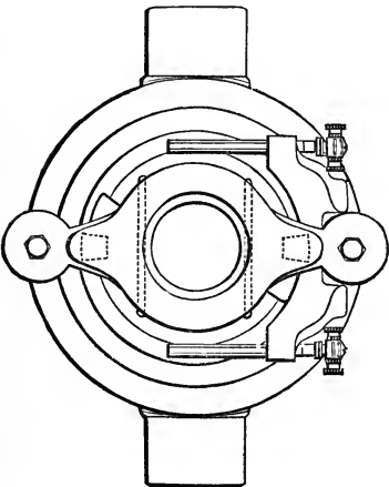
Fig. 21. Rear view.
