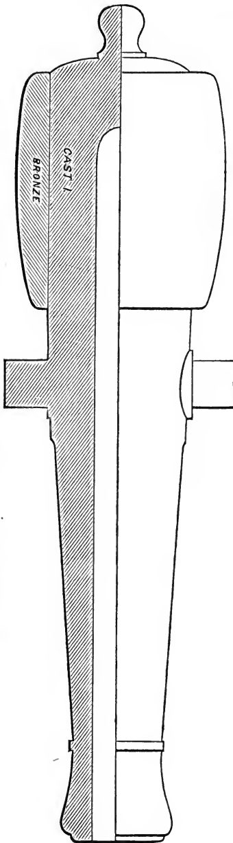
FIG. 59.—Attick's bronze reinforce. 100-pounder Scale \frac{5}{16} in. to 1 ft.
