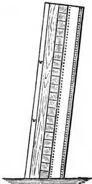
The Warrior target. Scale, \frac{1}{2} in. to 1 ft.
