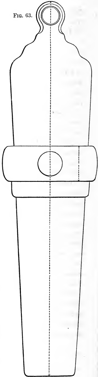
FIGS. 62, 63.—The Horsfall wrought-iron solid-forged 13-in. gun. Scale, \frac{1}{16} in to 1 ft.
