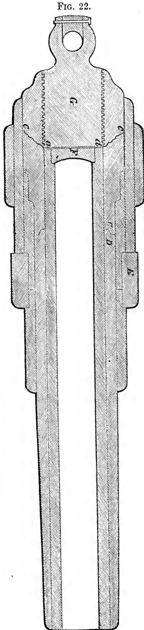
Armstrong 10\frac{1}{2} in. gun. \frac{1}{16} in. to 1 ft.
