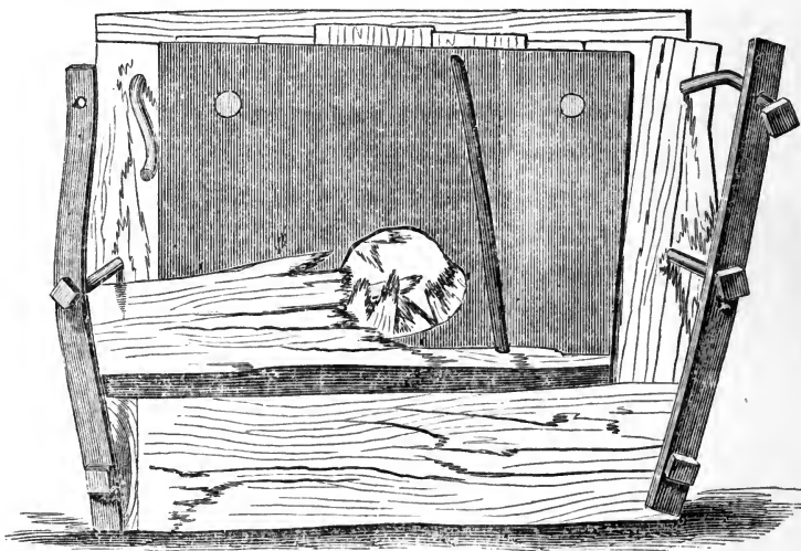
Front of 4\frac{1}{2} -in. plate, with 12-in. oak facing, after one 11-inch shot.
