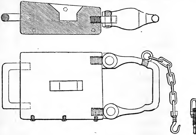
Cavalli breech-loader.
