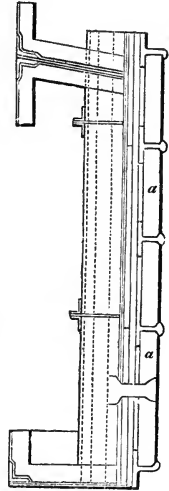
Scott Russell's target. Section. Scale, \frac{1}{4} in. to 1 ft.
