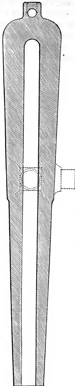
FIG. 71.—Krupp's 9-inch gun for Russia. Scale, \frac{1}{8} in. to 1 ft.
