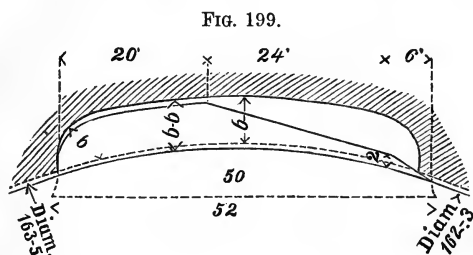
Present French groove and stud, Canon de 30 , full size.
