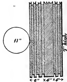
Ericsson 14-in. target.
