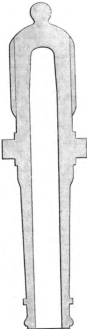
Blakely's 132-pounder of 1857. Scale, \frac{1}{10} in. to 1 ft.
