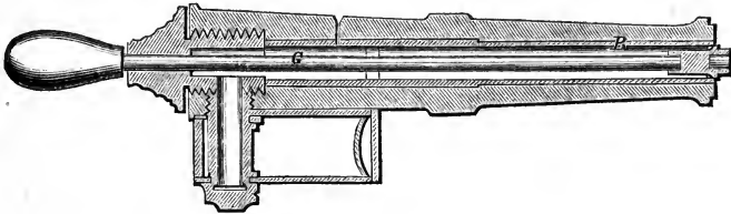
Adams's loading and cooling from the breech.
