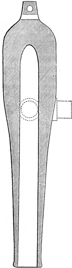
U. S. Navy 11-in. Dahlgren gun. Scale, \frac{1}{16} in. to 1 ft.
