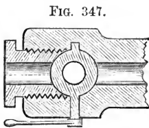
Alger's breech-loader.
