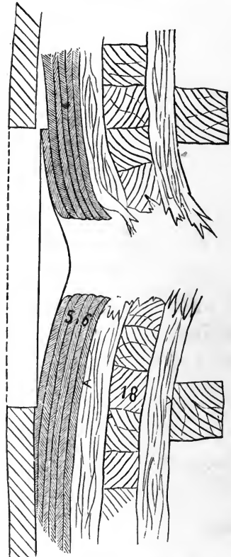
Section of 6\frac{1}{2} -in. laminated target.
