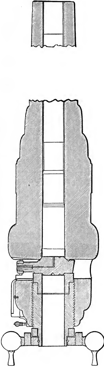
Fig. 340.—Section of breech of 110-pounder.
