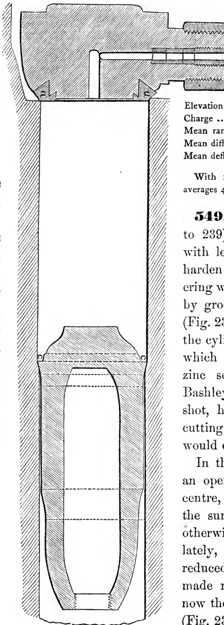
FIG. 236.—Chamber and projectile of 12-pounder. \frac{1}{2} size.
