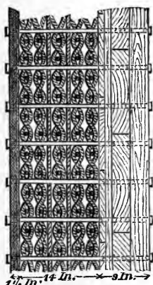
Section of wire target.
