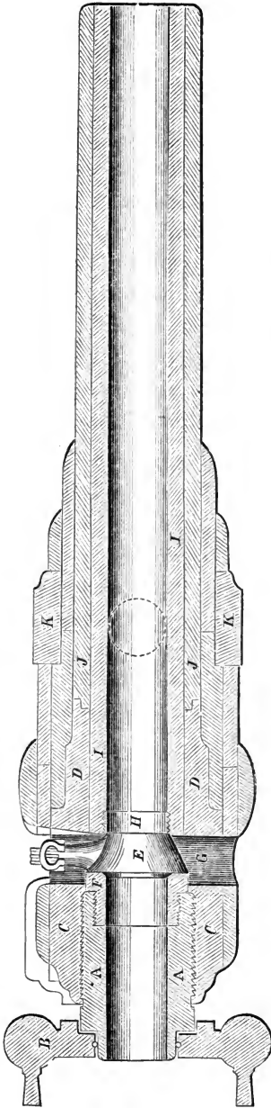
Fig. 344.—Longitudinal section of Armstrong 110-pounder. Scale, \frac{1}{16} in. to 1 ft.
