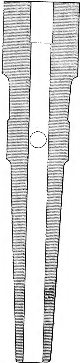
FIG. 69.—Section of Krupp's 9-inch solid steel gun in the Exhibition of 1862. Scale, \frac{1}{8} in. to 1 ft.
