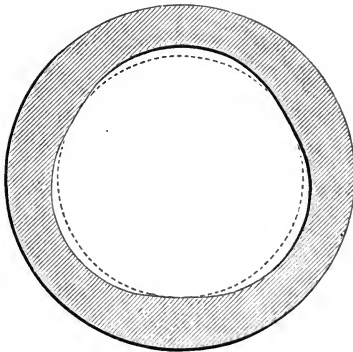
Haddan's rifling.
