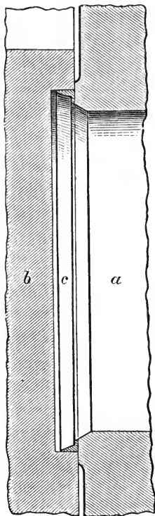
Krupp's gas-check.
