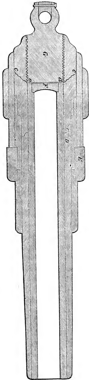
FIG. 177.—Armstrong 10½-in. muzzle-loader. Scale, \frac{1}{16} in. to 1 ft.
