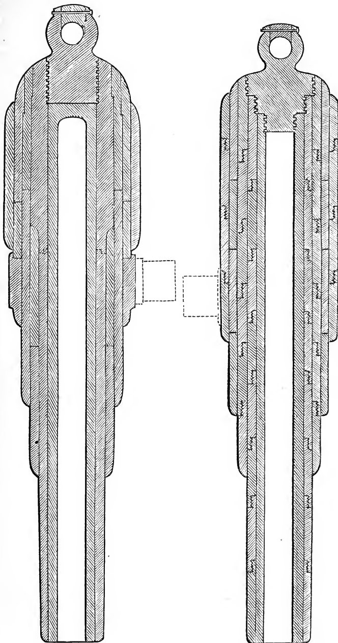
FIG. 27. 7-in. gun as built at Woolwich and rifled for Mr. Whitworth. Scale \frac{6}{17} in. to 1 ft.
