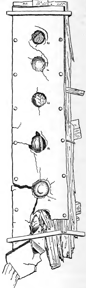
Nashua 4½-in. plate, after six 11-in. shot.
