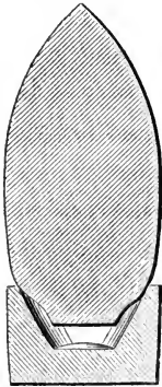
Timmerhaus's expanding shot.
