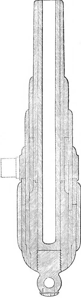
BRITISH STEEL-LINED COIL GUN.
