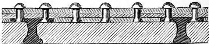
Section of Mr. Scott Russell's armor.
