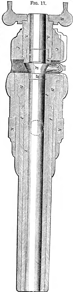
Armstrong 110-pounder. \frac{6}{10} in. to 1 ft.
