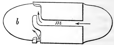
Bessemer's shot for smooth-bores.
