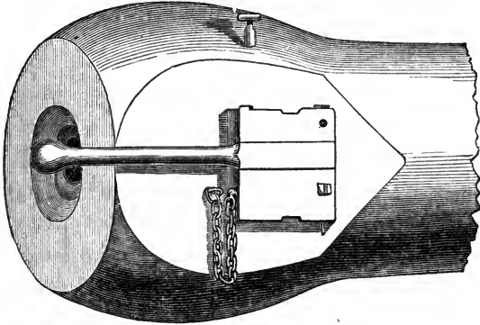
Breech of Krupp 110-pounder.
