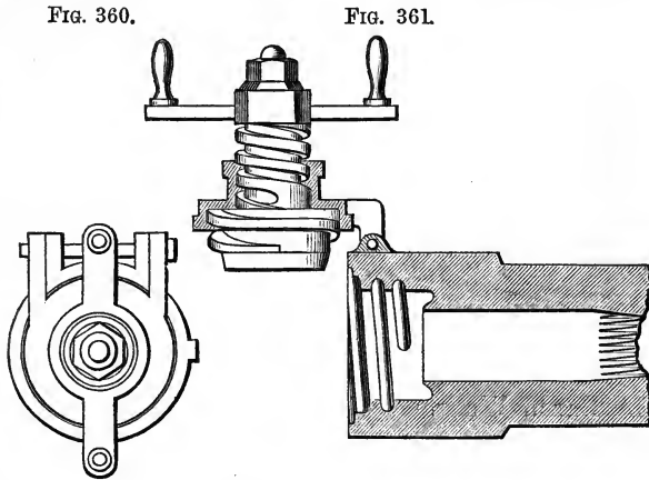
Screw breech-loader.
