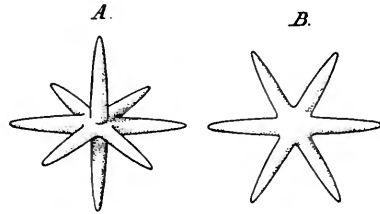
FIG. 95. Spicules of Astracospongia . A , octactine; B , hexactine. (After Hinde.)
