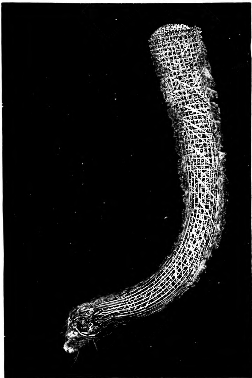
FIG. 15. Euplectella asperillum , Owen. (After Wyville Thompson.)
