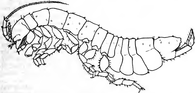
FIG. 119. Phreatoicus assimilis , ♀, from the side. × 8. (After Chilton.)
