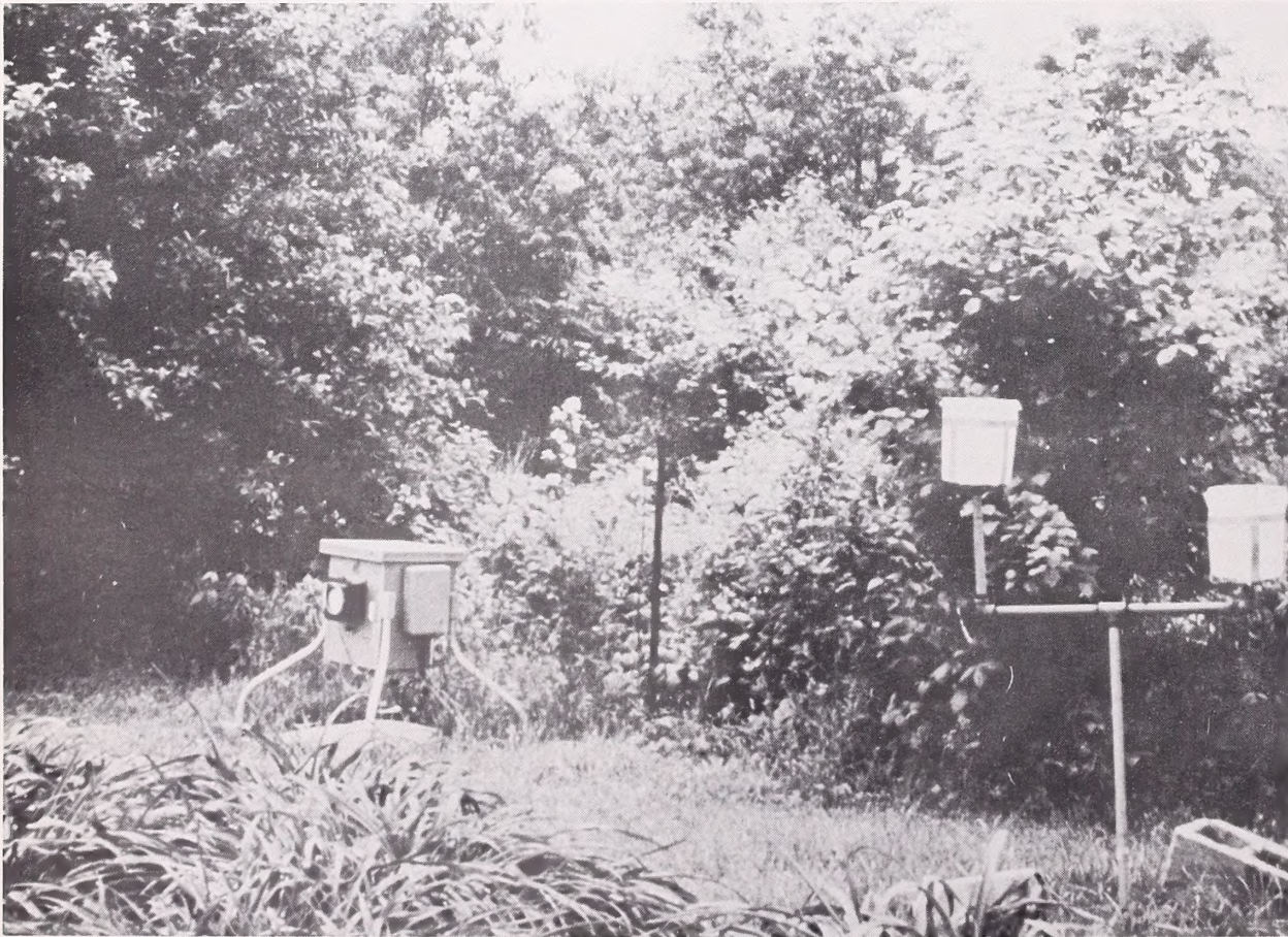
Aerial sampling for particulate pollutants is done with the dustfall bucket (lower right) for larger sizes of settling pollutants and with a Hi-Vol sampler for smaller particles, which tend to remain air-borne for indefinite periods. This set-up helps measure dustfall and suspended particles in an open area.
