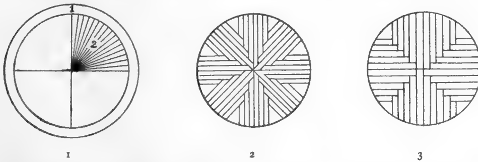
FIG. 1. (1) Sapwood; best taken off. (2) Feather-edged boards somewhat variable in width and thickness, but following the natural line of cleavage on the medullary rays of the wood.
