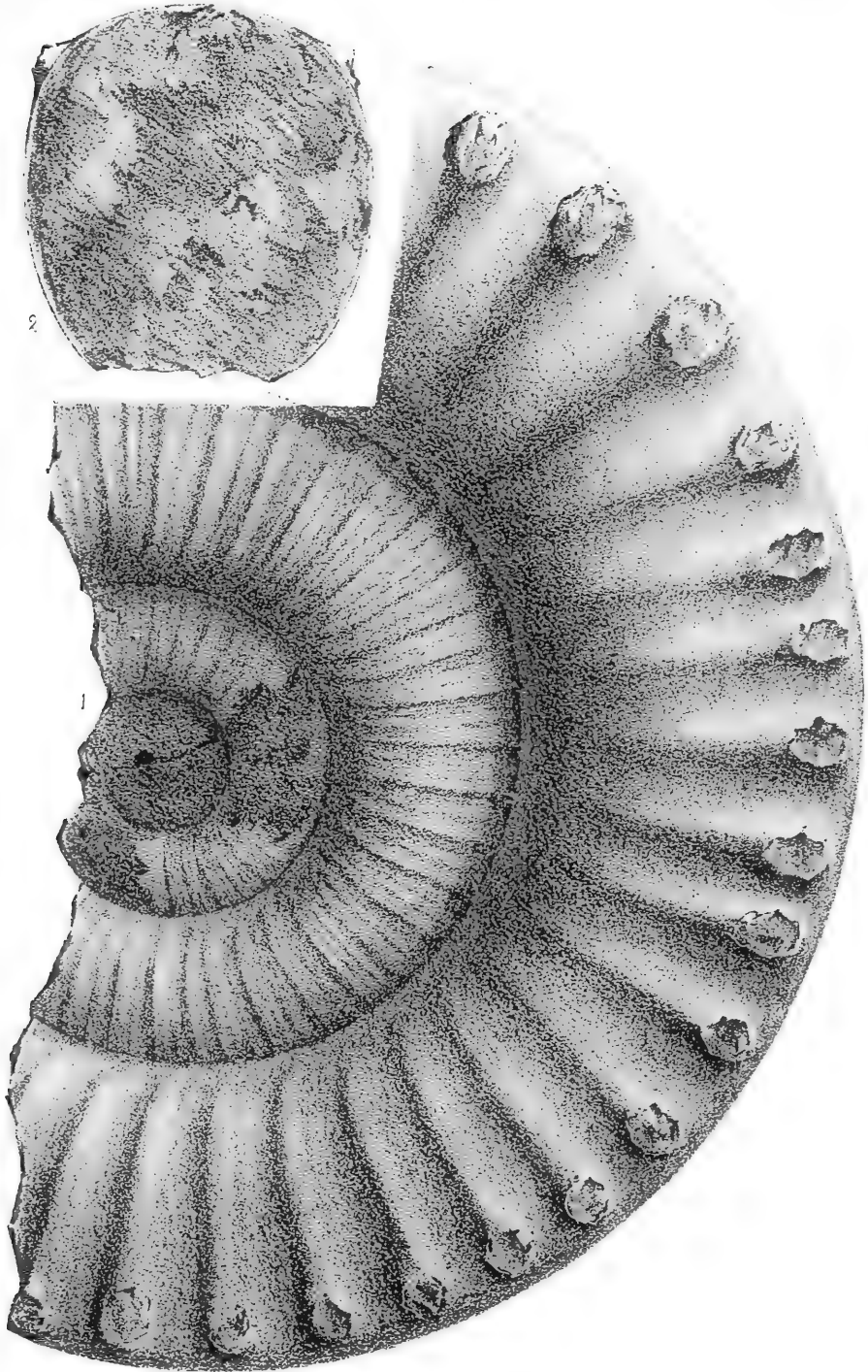
Ammonite (Fossil)
