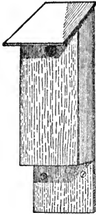
FIG. 2.—Sparrow-proof Box.
