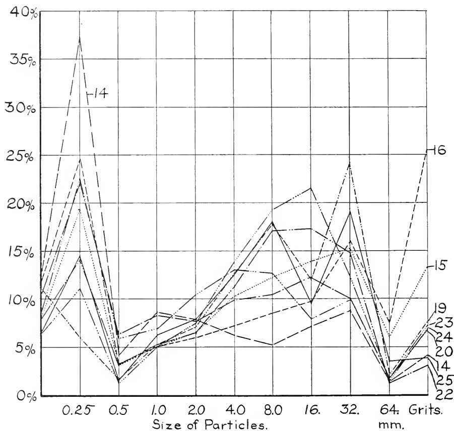
Fig. 4. Graph showing the results of the Hilgard elutriator method of mechanical analysis on the nine samples of Hanford fine sandy loam.
