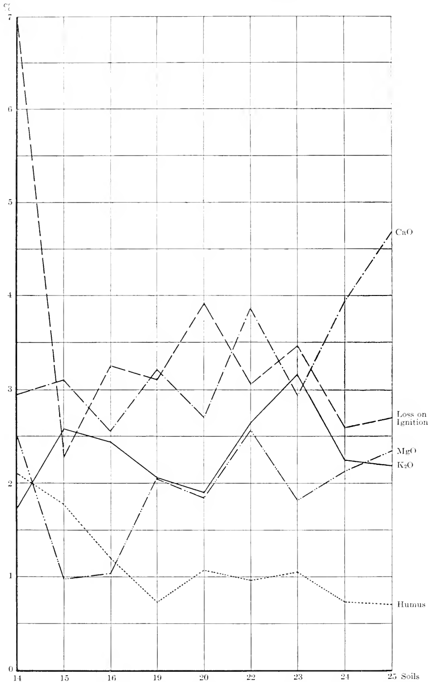
Fig. 18. Graph showing the loss on ignition, the amount of humus, and the percentages of calcium, magnesium, and potassium in the nine samples of Hanford fine sandy loam.
