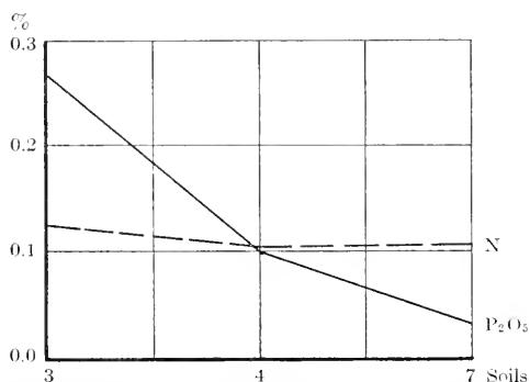
Fig. 12. Graph showing the percentages of nitrogen and of phosphorus in the three samples of Altamont clay loam.
