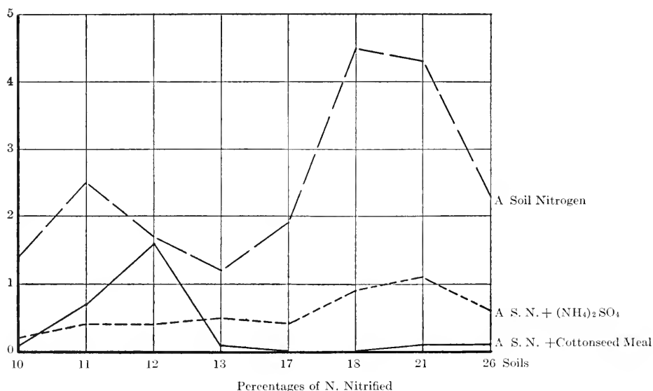
Fig. 25. Graph showing the percentages of nitrogen in various nitrogen containing materials nitrified in the eight samples of the San Joaquin sandy loam.
