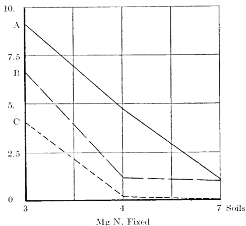
Fig. 20B. Graph showing nitrogen fixation in milligrams in the three horizons of the three samples of Altamont clay loam.
