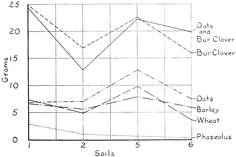
Fig. 27. Graph showing the total dry matter produced by wheat, barley, oats, Phaseolus , bur clover, and oats and bur clover on the four samples of Diablo clay adobe. First crop.
