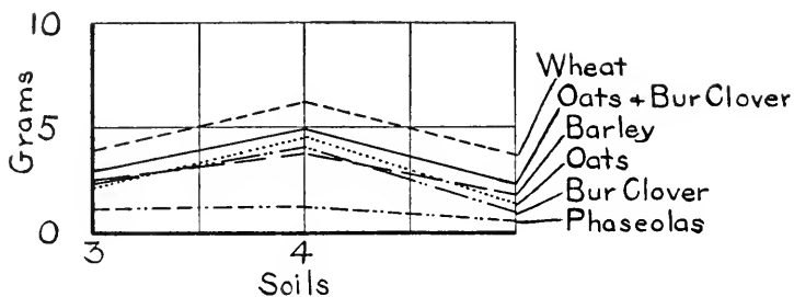
Fig. 29. Graph showing the total dry matter produced by wheat, barley, oats, bur clover, Phaseolus , and oats and bur clover on the three samples of Altamont clay loam. First crop.
