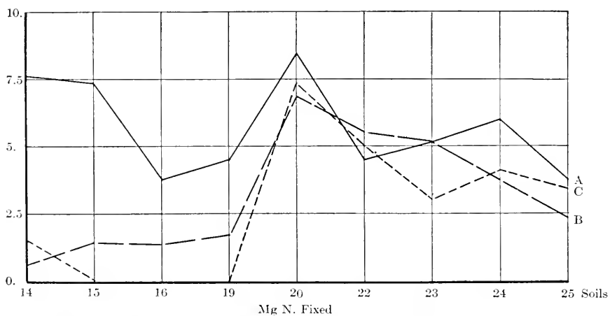
Fig. 22B. Graph showing nitrogen fixation in the three horizons of the nine samples of Hanford fine sandy loam.
