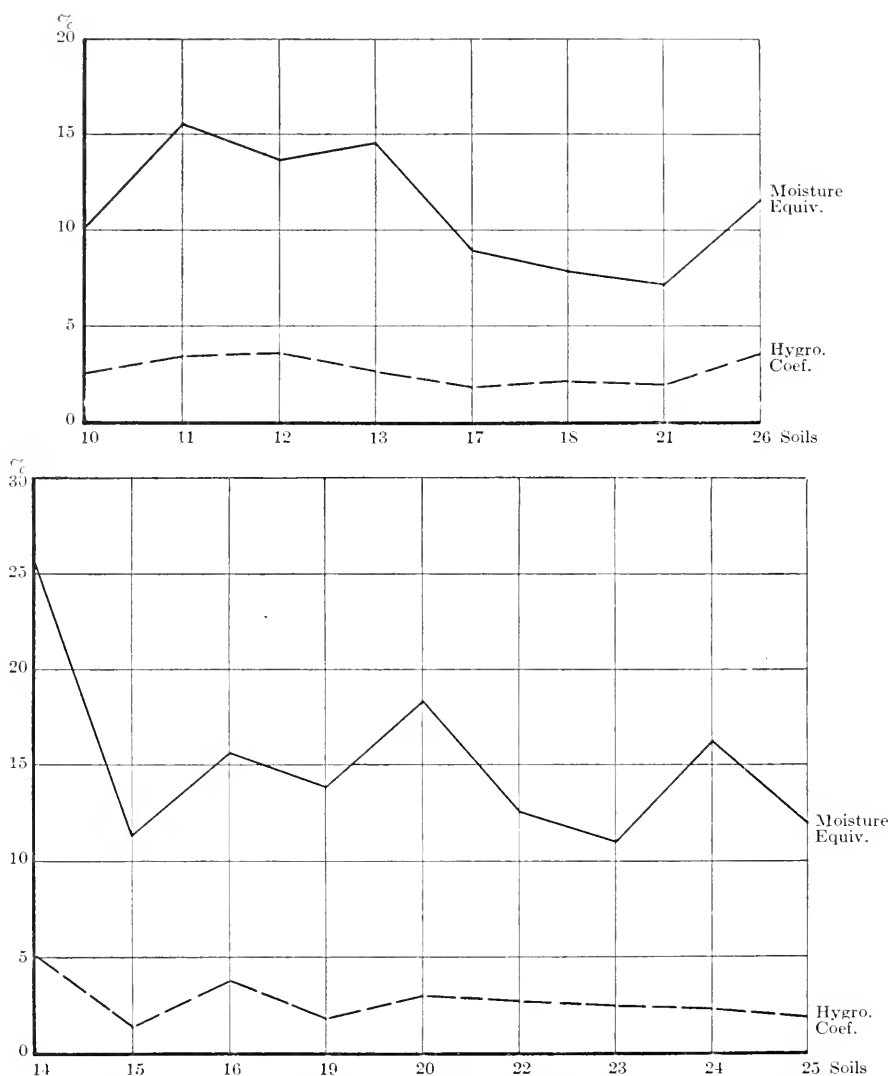
Fig. 10. Graph showing the results of the determination of the moisture equivalent and of the hygroscopic coefficient on the eight samples of San Joaquin sandy loam and the nine samples of Hanford fine sandy loam.
