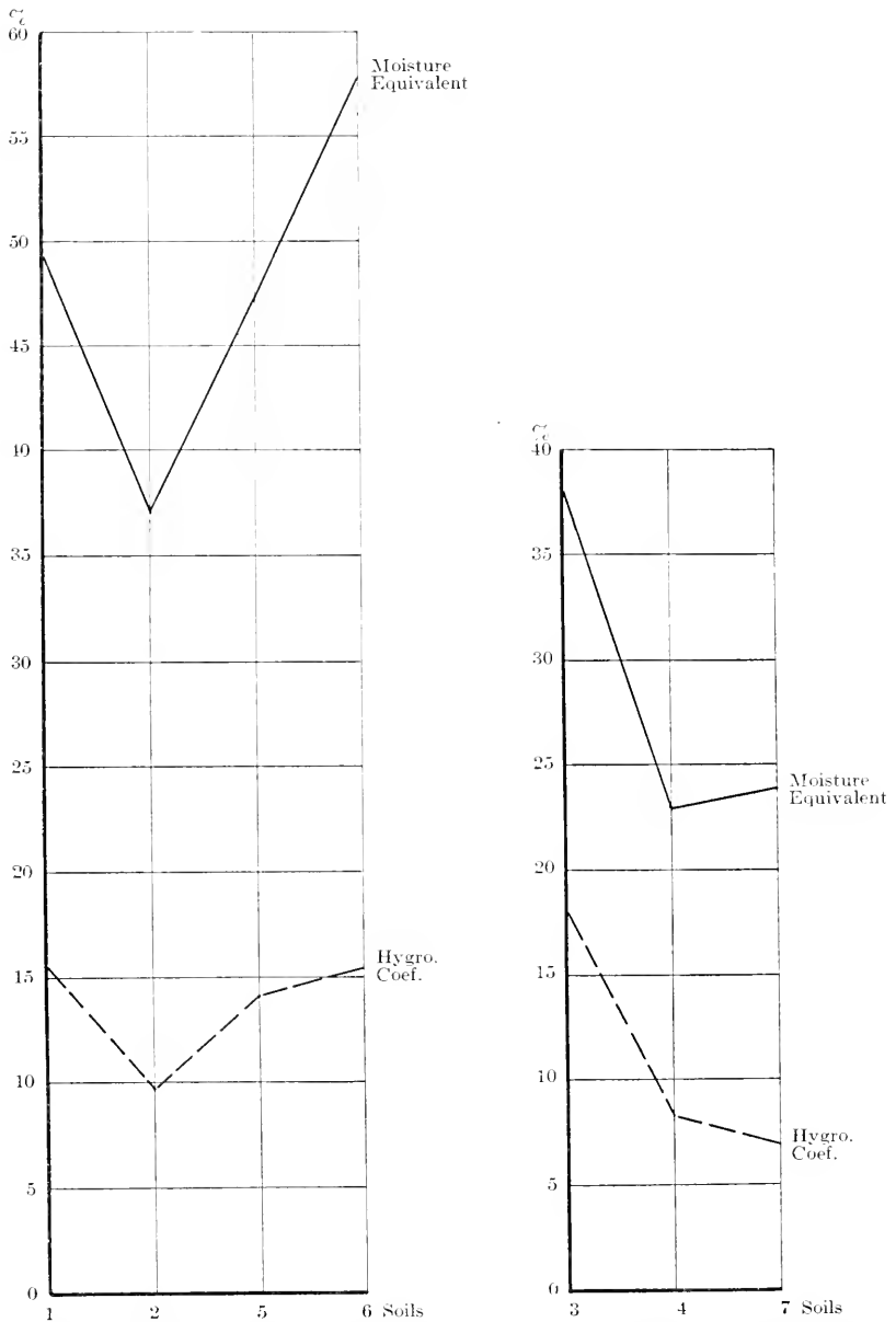
Fig. 9. Graph showing the results of the determination of the moisture equivalent and of the hygroscopic coefficient on the four samples of Diablo clay adobe and the three samples of Altamont clay loam.
