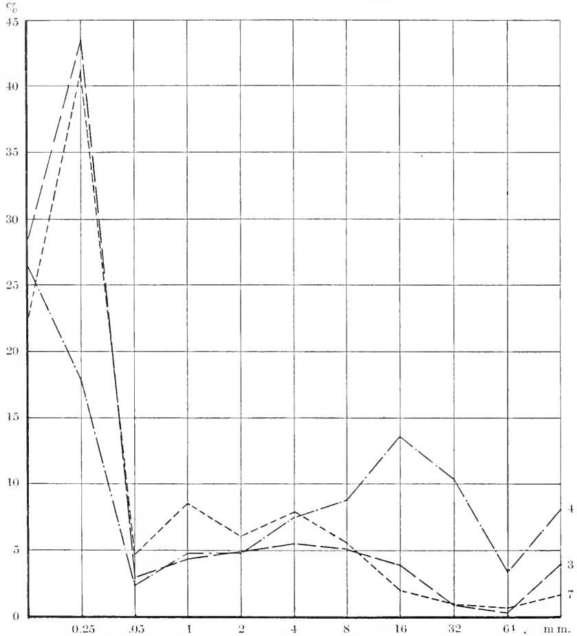
Fig. 2. Graph showing the results of the Hilgard elutriator method of mechanical analysis on the three samples of Altamont clay loam.
