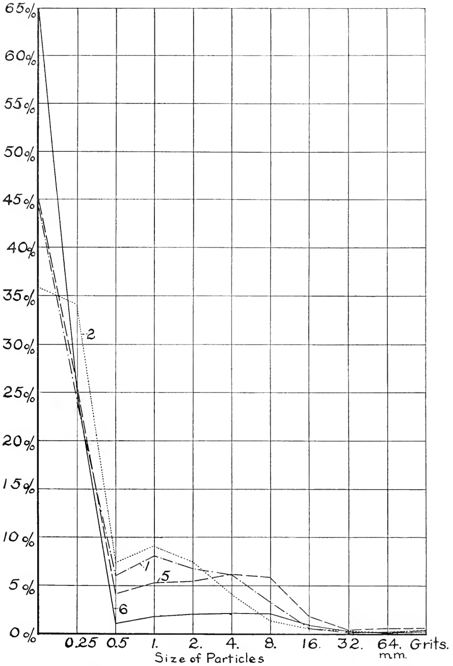
Fig. 1. Graph showing the results of the Hilgard elutriator method of mechanical analysis on the four samples of Diablo clay adobe.
