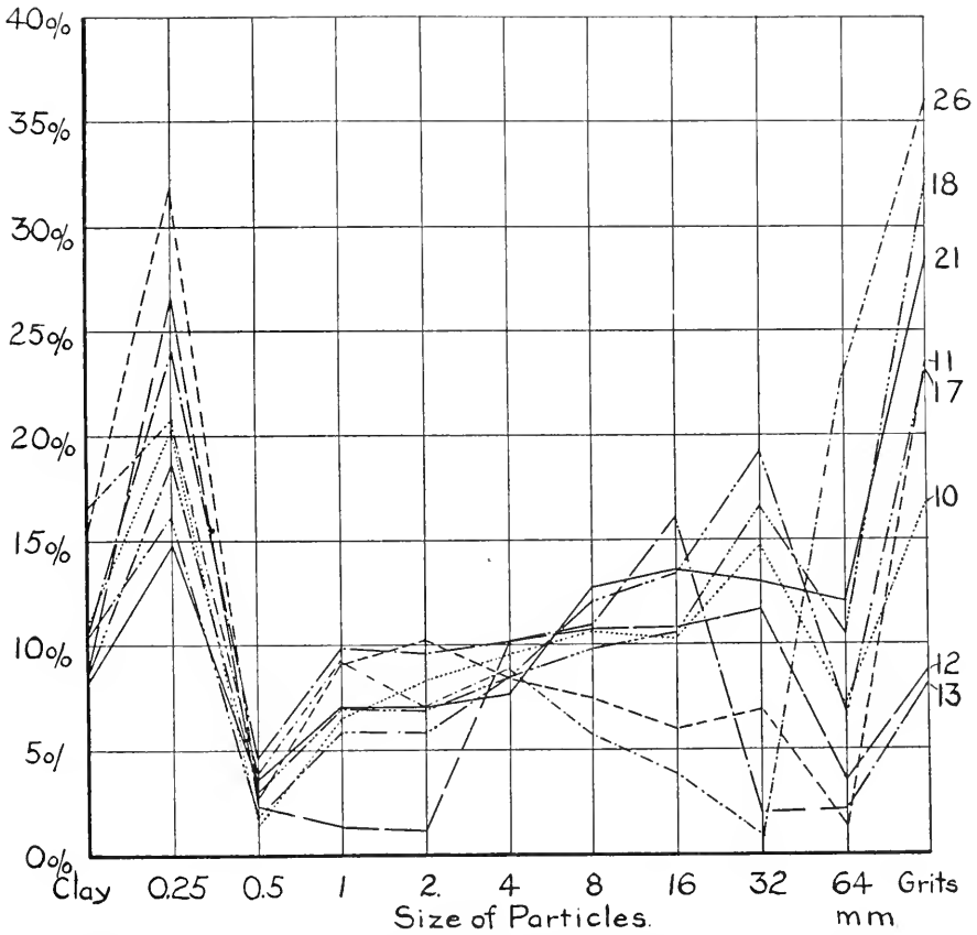
Fig. 3. Graph showing the results of the Hilgard elutriator method of mechanical analysis on the eight samples of San Joaquin sandy loam.
