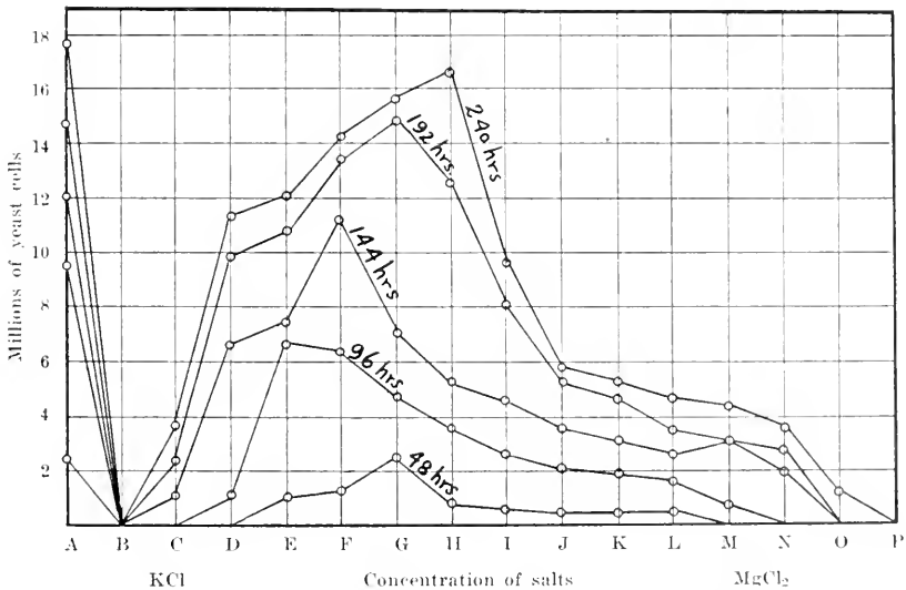
Fig. 10.—Curves of yeast growth showing antagonism between KCl and MgCl_2 . The ordinates represent the number of yeast cells in millions and the abscissae, the concentration of salts in combination. The ordinate at A represents the number of cells in blank cultures.
