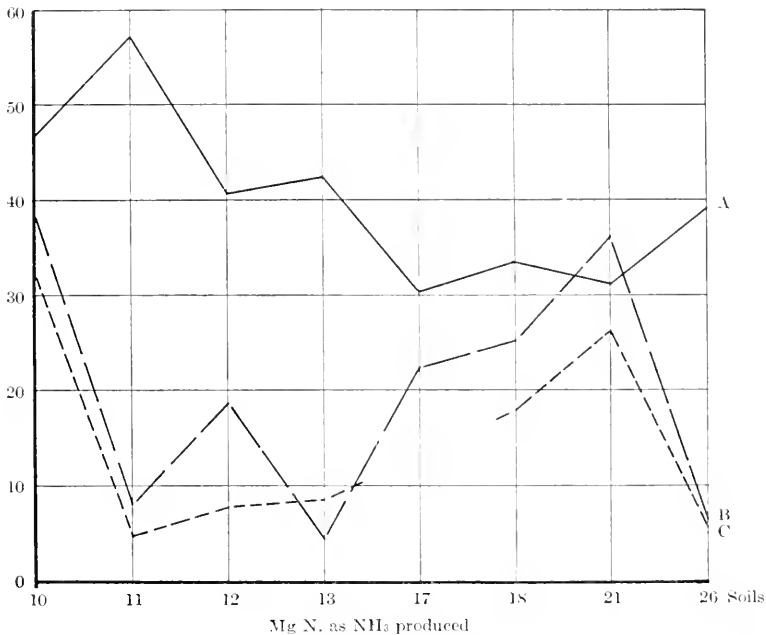
Fig. 21A. Graph showing ammonification in the three horizons of the eight samples of San Joaquin sandy loam.
