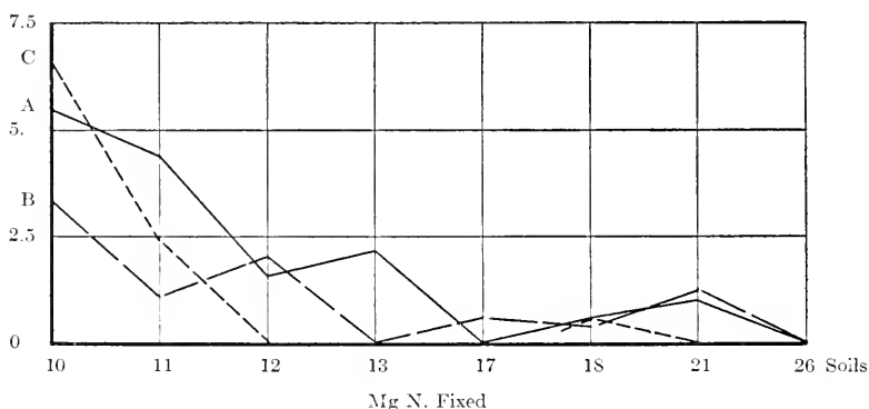
Fig. 21B. Graph showing nitrogen fixation in the three horizons of the eight samples of San Joaquin sandy loam.
