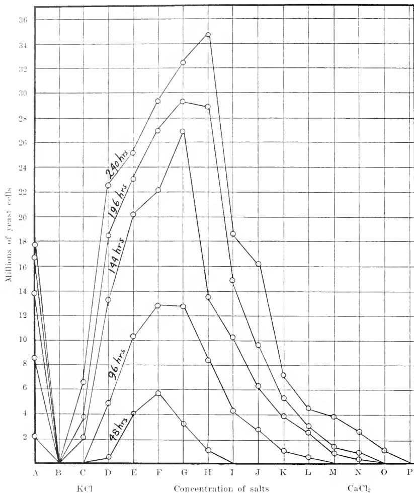
Fig. 7.—Curves of yeast growth showing antagonism between KCl and CaCl 2 . The ordinates represent the number of yeast cells in millions and the abscissae, the concentration of salts in combination. The ordinate at A represents the number of yeast cells in blank cultures.
