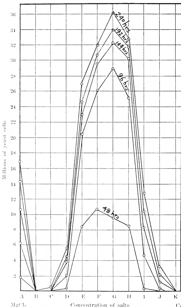
Fig. 6.—Curves of yeast growth showing antagonism between MgCl_2 and CaCl_2 . The ordinates represent the number of yeast cells in millions and the abscissae, the concentration of the salts in combination. The ordinates at A represent the number of yeast cells in blank cultures.
