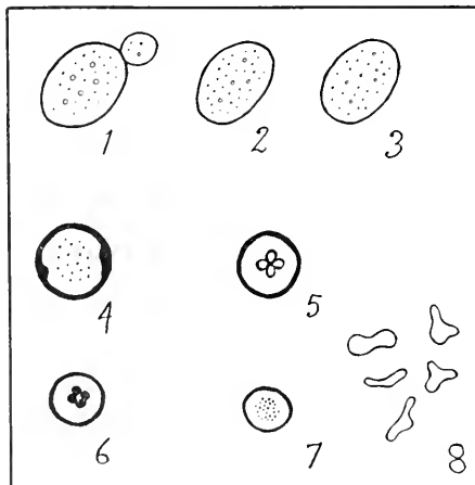
Fig. 5c.—Appearance of yeast cells in extreme concentrations of salts. Normal yeast cells in 1, 2 and 3, diseased yeast cells from extreme concentrations of KCl and MgCl 2 in 4 and 5; (white) and diseased yeast cells from extreme concentrations of CaCl 2 and NaCl in 6, 7 and 8 (black or shadowy) (X5000).
