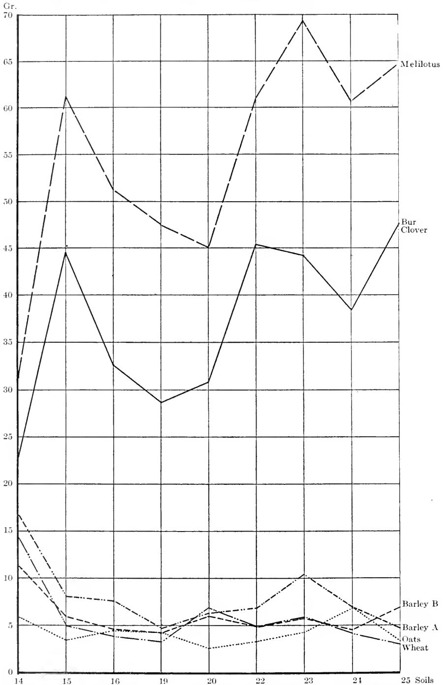
Fig. 33. Graph showing the total dry matter produced by wheat, oats, barley (two series), bur clover, and Melilotus indica on the nine samples of Hanford fine sandy loam. Second crop.
