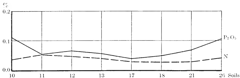
Fig. 13. Graph showing the percentages of nitrogen and of phosphorus in the eight samples of San Joaquin sandy loam.
