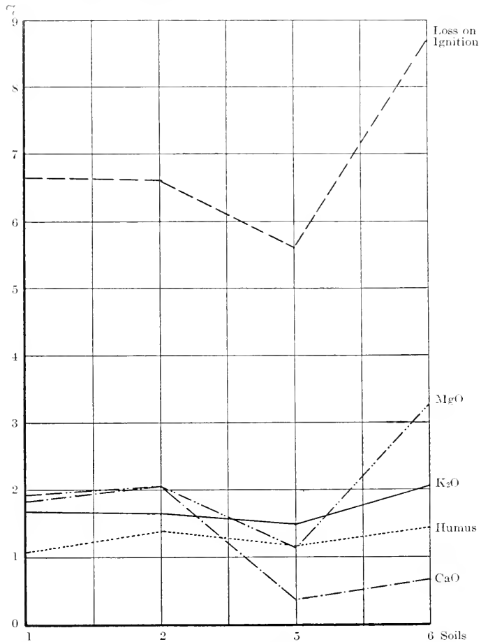
Fig. 15. Graph showing the loss on ignition, the amount of humus, and the percentages of calcium, magnesium, and potassium in the four samples of Diablo clay adobe.
