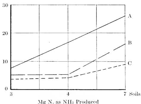
Fig. 20A. Graph showing ammonification in the three horizons of the three samples of Altamont clay loam.
