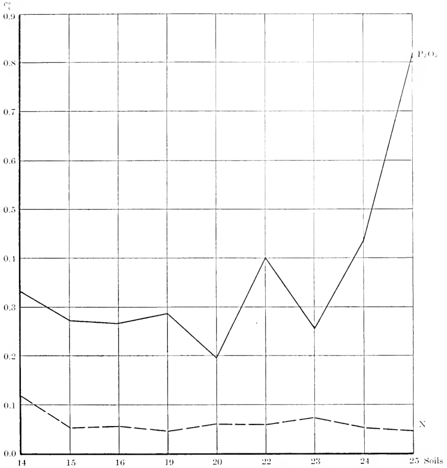
Fig. 14. Graph showing the percentages of nitrogen and of phosphorus in the nine samples of Hanford fine sandy loam.
