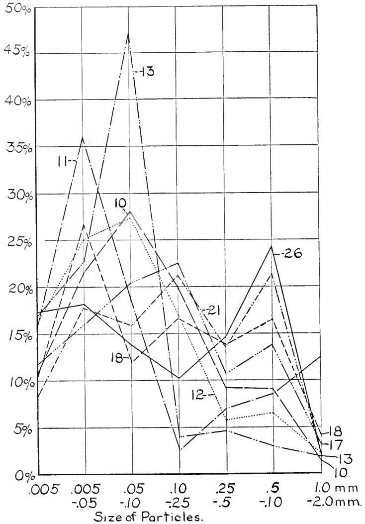
Fig. 7. Graph showing the results of the Bureau of Soils method of mechanical analysis on the eight samples of San Joaquin sandy loam.
