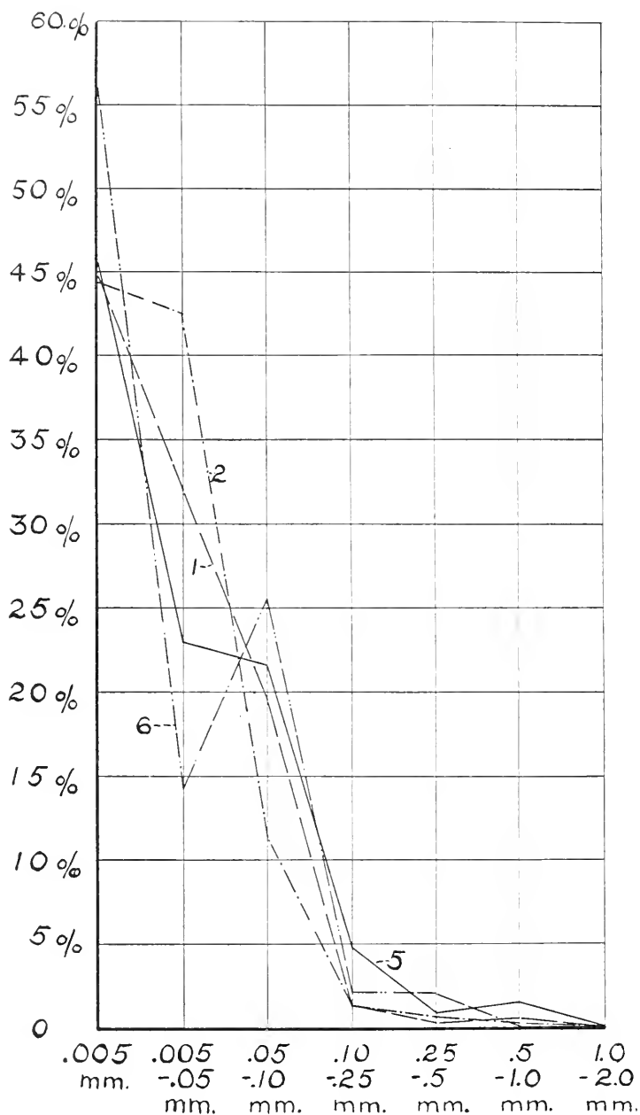
Fig. 5. Graph showing the results of the Bureau of Soils method of mechanical analysis on the four samples of Diablo clay adobe.
