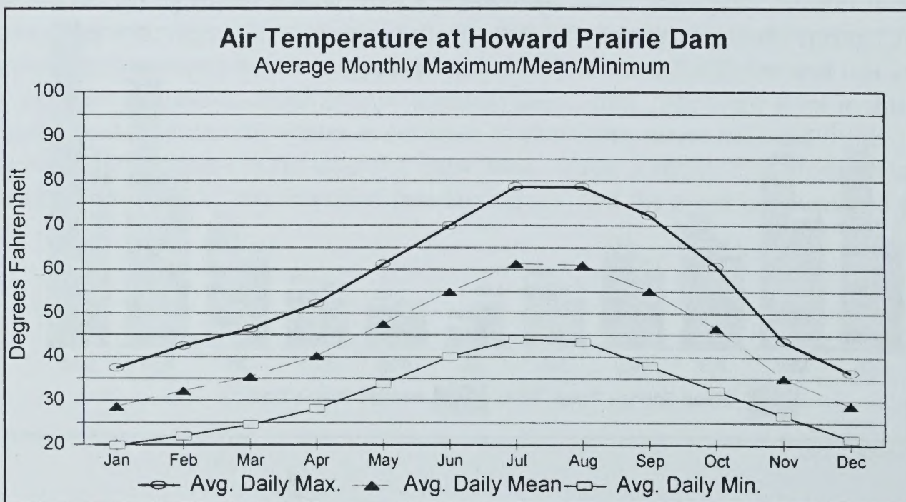
Figure 3. Air Temperature at Howard Prairie Dam NOAA Station (1961-1998)
