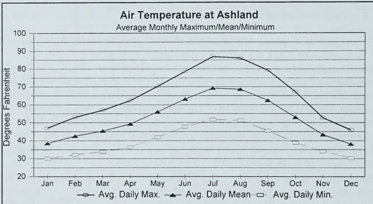
Figure 2. Air Temperature at Ashland NOAA Station (1961-1998)
