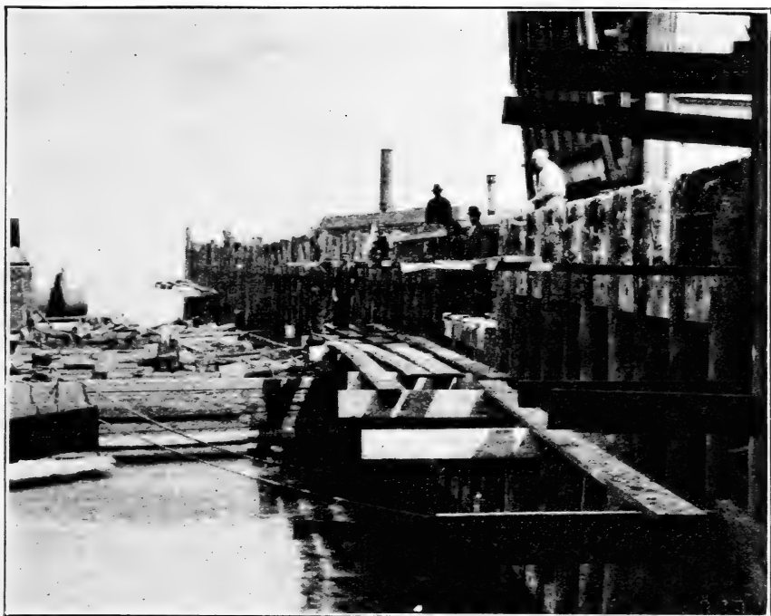
FIG. 6.—A ferry slip, San Francisco, Cal., constructed of blue-gum piles.
