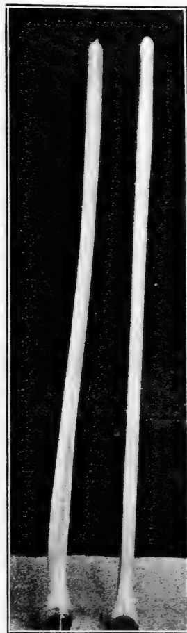
FIG. 7.—Blue-gum (crooked) and hickory (straight) ax helves. Blue-gum helve cut from plank air-seasoned for two years.
