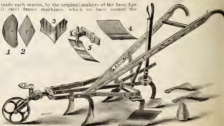
Fig. 1, Rounded Teeth; Fig. 2, Diamond Teeth; Fig. 3, Rear Plow; Fig. 4, Side Hoe; Fig. 5, Weeder; Fig. 6, Wheel; Fig. 7, Horse Hoe ready for operation.
