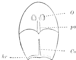
Figur 8. Didymaspis Grindrodi . E. R. LANKESTER. LOWER Old Red Sandstone von Ledbury, Herefordshire in England. Oberes Kopfschild. O = Augenöffnung, po = Parietalorgan, Co = Crista occipitalis , hr = Hinterrand. (Nach RAY LANKESTER.)
