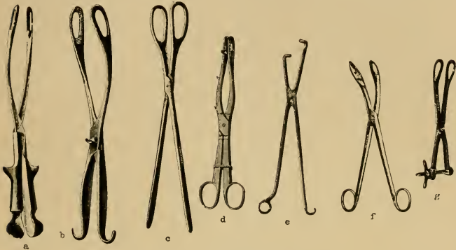
FIG. 93. OBSTETRIC FORCEPS.
