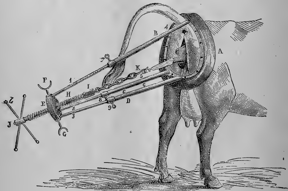
Fig. 57. OBSTETRIC MACHINE. z
