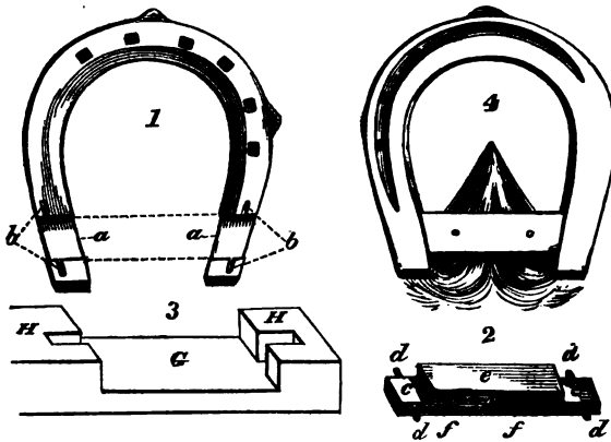
Fig. 1 represents the shoe prepared for the reception of the vulcanized rubber.
