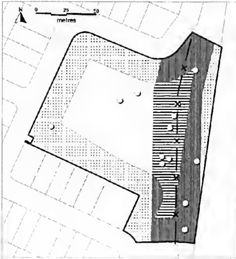
Fig. 1. Amberfield Grassland Reserve showing twenty metre buffers from perimeter (light shading), internal fence (horizontal hatching) and overlap (dark shading), with locations of Golden Sun Moth observations in 2015 (open circles).
