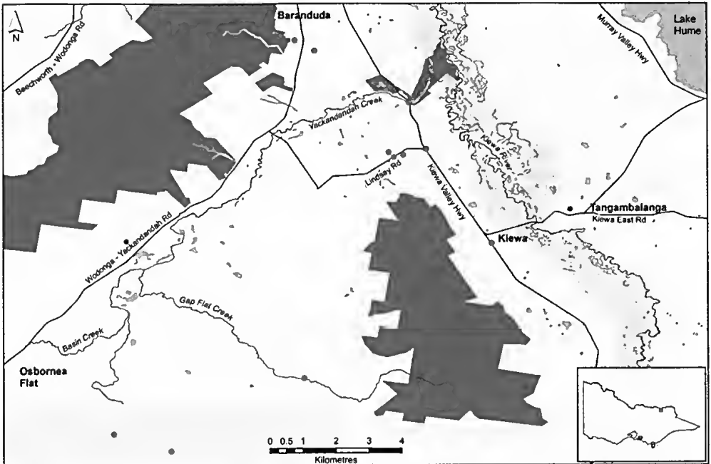
Fig. 1. Location of Eastern Dwarf Tree Frog Litoria fallax sightings (red dots) in north-east Victoria.
