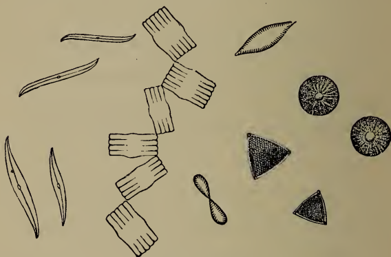
FIG. 26.— Diatoms.
