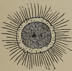
FIG. 19.— Actinosphaerium eichornii .
