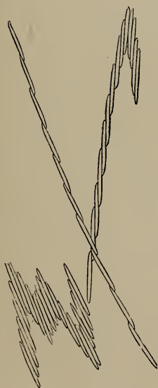
FIG. 27.— Bacillaria Paradoxa .
