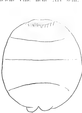
Fig. 31. — Callidina spec.
