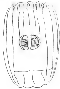
Fig. 32. — Callidina spec.
