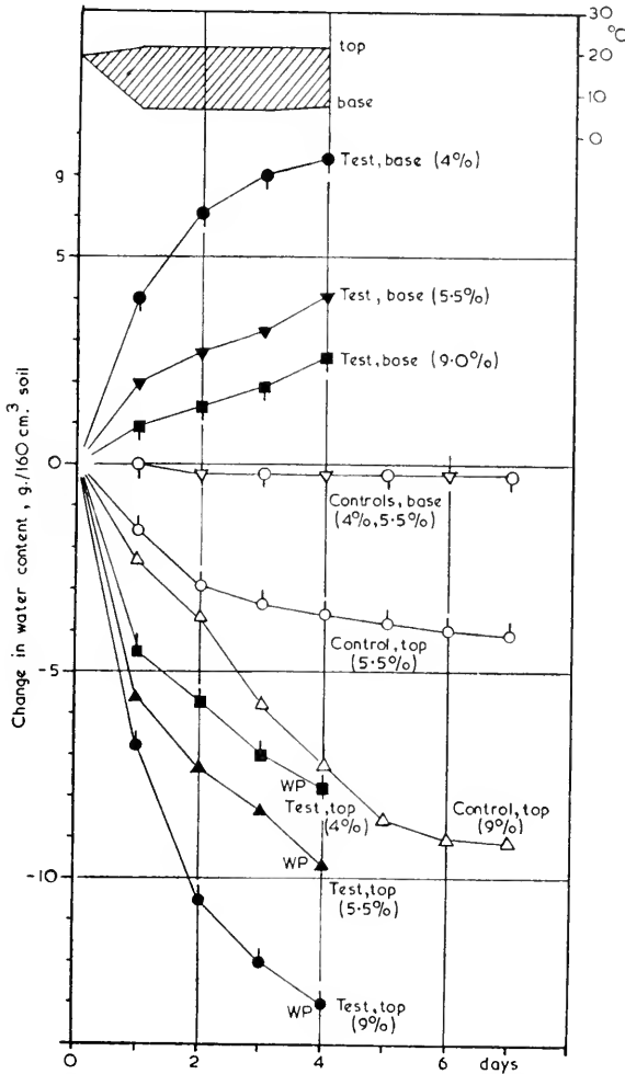
FIG. 7. Ecological effect of an inverse temperature gradient on the vapour movement and condensation in soils of different moisture, with rooted plants. For key, see Fig. 3. Vapour tension of air: 60%.
