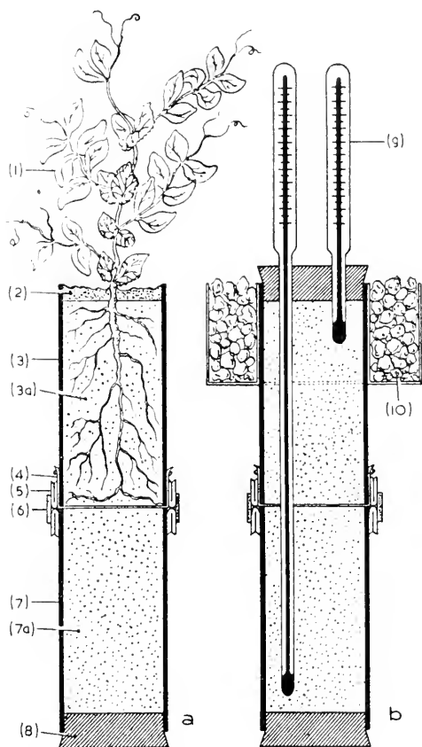
FIG. 1. Test equipment, (a) with test plants, (b) without test plants, apical containers enclosed in ice jacket. Key: (1) Test plant, (2) Petroleum jelly-vaseline sealing, (3) Glass wall of the apical tube, (3a) Apical soil column (= 'top'), (4) Perlon diaphragm, (5) Folded rubber hose, (6) Strip of plaster, (7) Glass wall of the basal tube, (7a) Basal soil column (= 'base'), (8) Rubber plugs, (9) Thermometers, (10) Hollow cylindrical ice containers.
