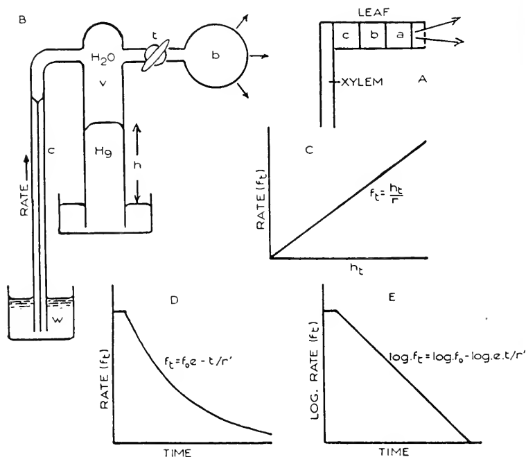
FIG. 1. A: Diagrammatic representation of a train of mesophyll cells. B: Model of transpiring cell on the hypothesis that the water moves through the vacuoles. v , vacuole; c , capillary tube; w , reservoir of water; t , tap; b , porous bulb. C, D and E: Graphs showing the characteristics of the die-away curve of uptake by the vacuole when the tap t is closed.
