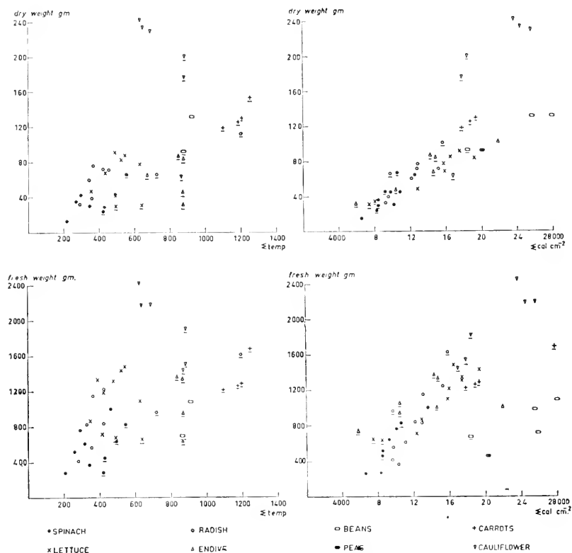
FIG. 3. The effect of heat- and radiation-sum on dry- and fresh-weight yield per container of various vegetables. The data obtained in autumn are underlined.
