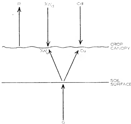
FIG. 2. Heat balance of crop canopy. For symbols, see text.
