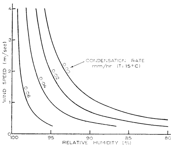
FIG. 1. Condensation on horizontal leaf for given wind speed and relative humidity, calculated from eq. 4.
