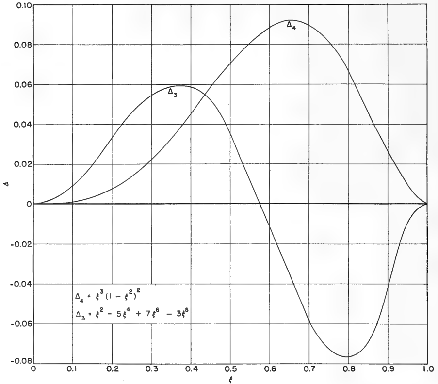
Figure 13 - Distribution Functions Following Equations [6a] and [6b]
