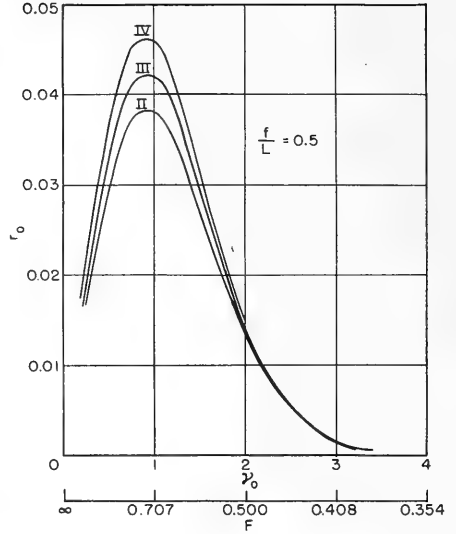
Figure 18 - Total Wave-Resistance Coefficients r_0 of the TMB
