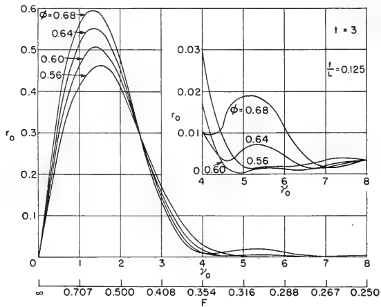
Figure 31 - Wave-Resistance Coefficients r_0 = \frac{R}{4\pi C^2 \rho g b^4/a} , of Symmetrical Bodies Belonging to the Class (2,4,6;\phi;t) = 1 - a_2 \xi^2 - a_4 \xi^4 - a_6 \xi^6 Over \gamma_0 = 1/2F^2 and F = U/\sqrt{gL} t = 3
