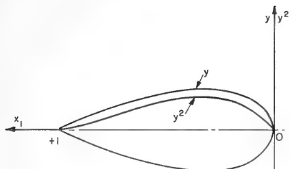
Figure 3a - Landweber's Axes
