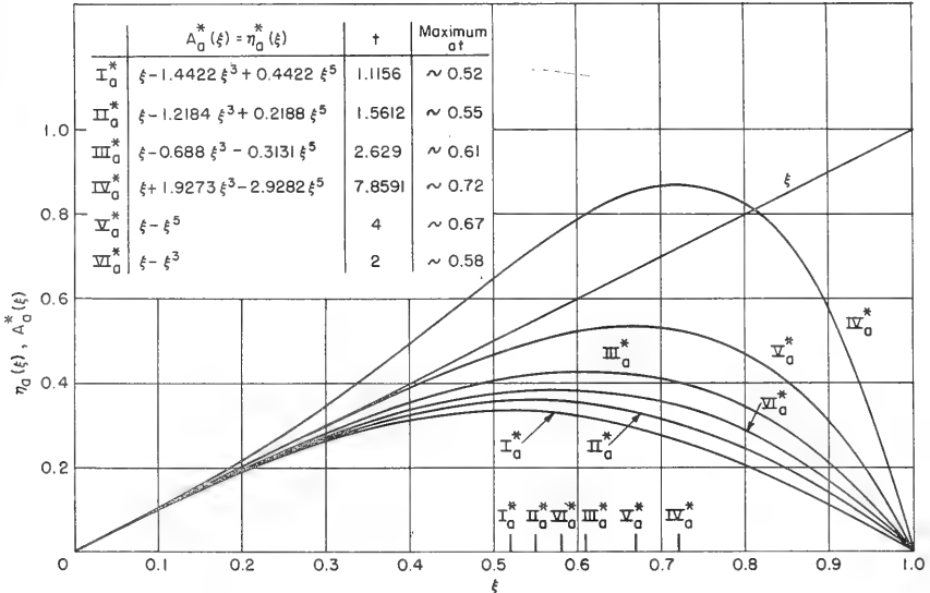
Figure 5 - Examples of the Antisymmetrical (Skew) Parts of Sectional-Area Curves A_a^*(\xi) (Doublet Distributions \mu_a^*(\xi) ) Belonging to the Family \xi + b_3 \xi^3 - (1 + b_3) \xi^5
