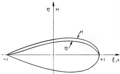
Figure 3b - Present Axes
