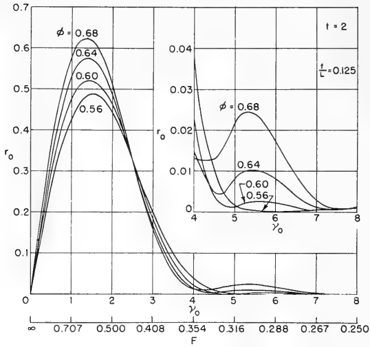
Figure 30 - Wave-Resistance Coefficients r_0 = \frac{R}{4\pi C^2 \rho g b^4/a} , of Symmetrical Bodies Belonging to the Class (2,4,6;\phi;t) = 1 - a_2 \xi^2 - a_4 \xi^4 - a_6 \xi^6 Over \gamma_0 = 1/2F^2 and F = U/\sqrt{gL} t = 2
