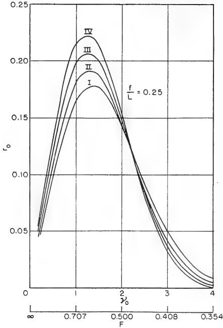
Figure 17 - Total Wave-Resistance Coefficients r_0 of the TMB Models Shown in Figures 14 and 15, f/L = 0.25
