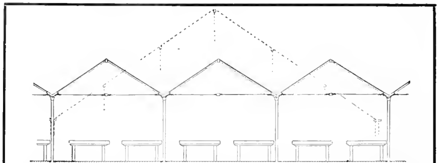
View of a piece of ground 40 ft. respectively 41 ft. 6 in. in width, covered by one roof (old style), and also by three sections of our Patent "Short-Roof" Construction. Compare headroom over benches and number of supports.
