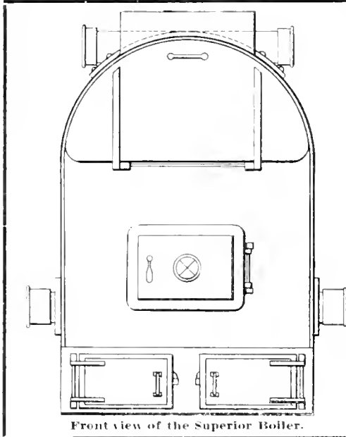
Front view of the Superior Boiler.
