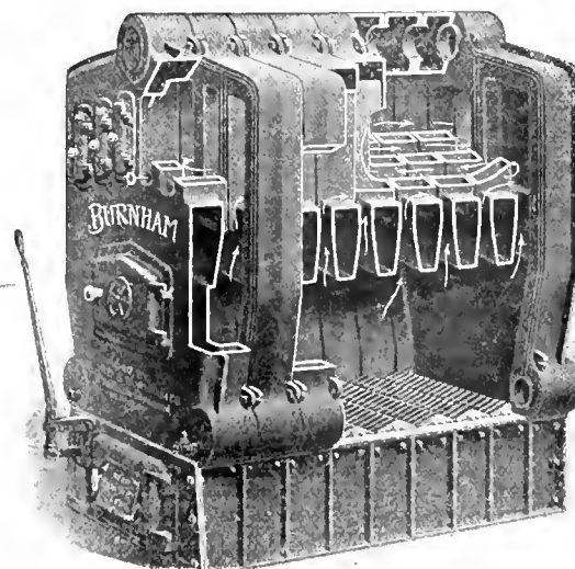
"BURNHAM" BOILERS.
