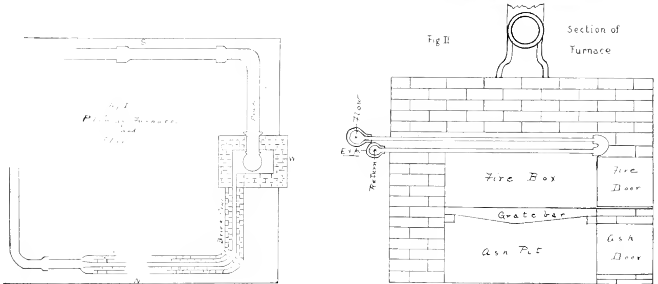
Plan for Furnace and Flue with Hot Water Coil in Fire Box.
