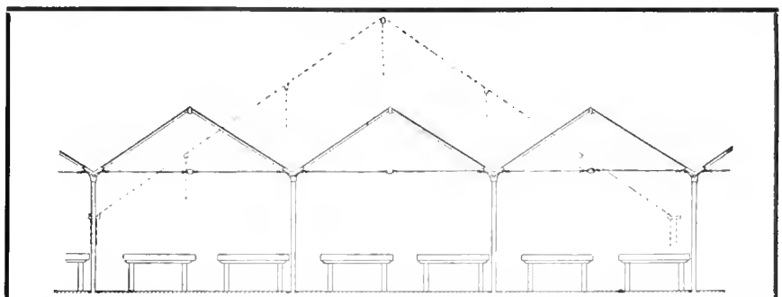
View of a piece of ground 40 ft. respectively 41 ft. 6 in. in width, covered by one roof (old style), and also by three sections of our Patent "Short-Roof" Construction. Compare headroom over benches and number of supports.
