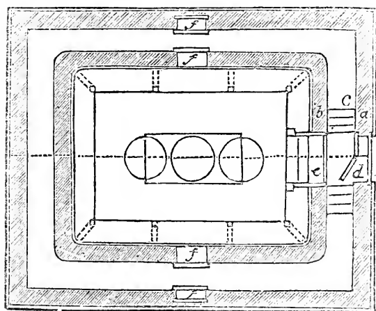
Fig. 24. Ground Plan of a Fruit Room.
