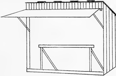
OPEN-FRONT COLONY HOUSE WITHOUT SCRATCHING SHED.
