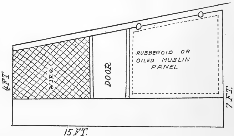
HOFFMAN'S COMBINATION OPEN-FRONT HOUSE AND SCRATCHING PEN
