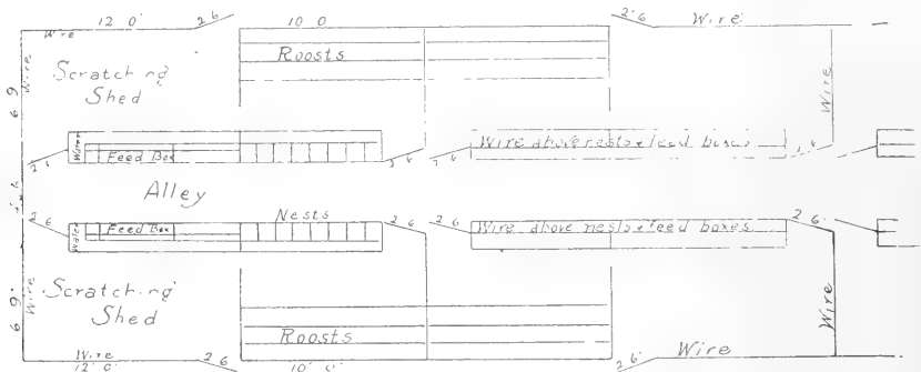
W. G. SUITS' GROUND PLAN OF DOUBLE HOUSES, BANDINI RANCH, RIVERSIDE, CAL.
