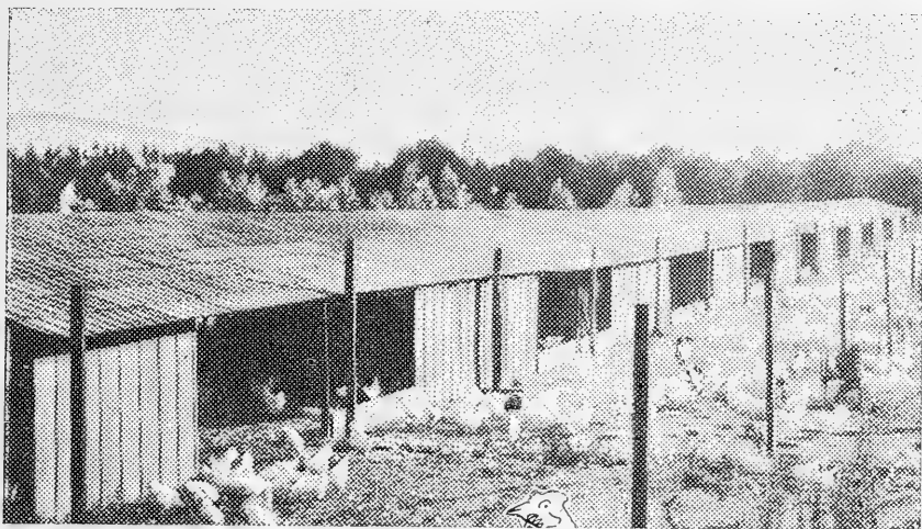
CONTINUOUS HOUSE AND SCRATCHING SHED.
