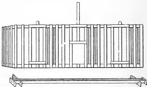
THREE-COMPARTMENT FATTENING COOP AND TROUGH.
