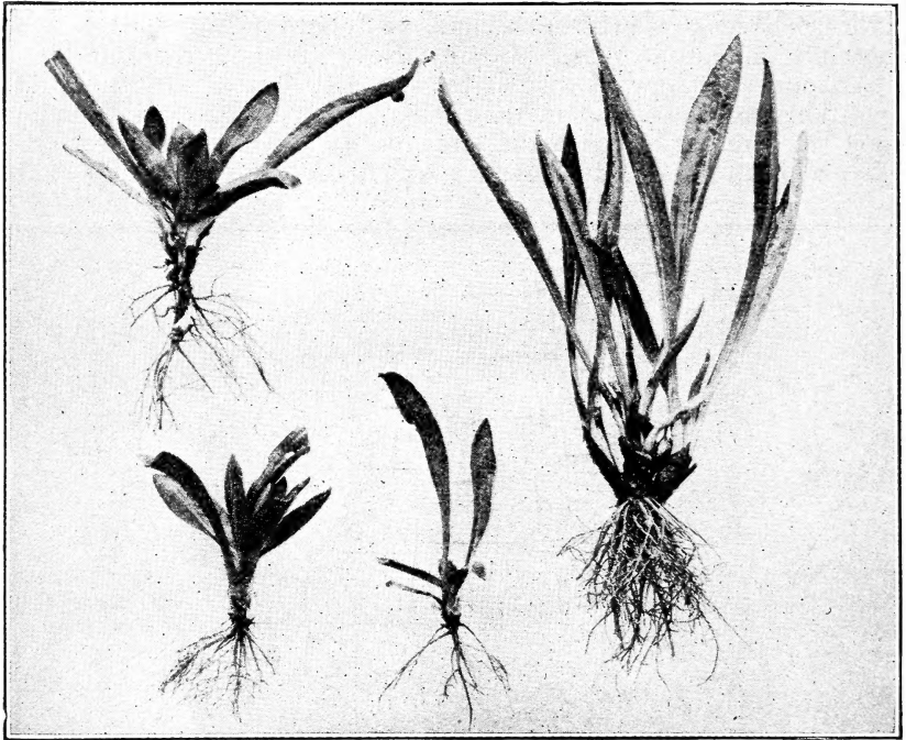
FIG. 3.— Helinium hoopesii . Young plants showing root system and method of vegetative reproduction.
