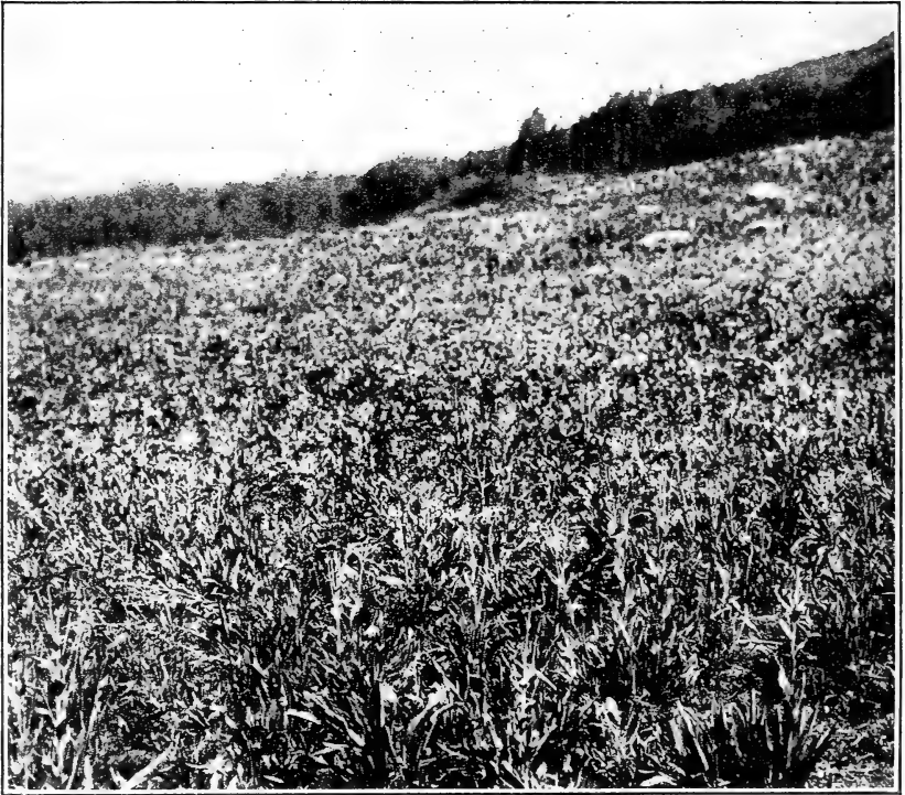
FIG. 4.—An overgrazed range on which Helonium hoopesii has taken almost complete possession.
