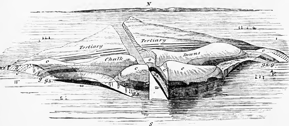
Fig. 19.—Diagram illustrative of the geological structure of the Isle of Wight. c , Upper and Lower chalk; f , Upper Greensand; g , Gault; s , Lower Greensand; w , Wealden.
