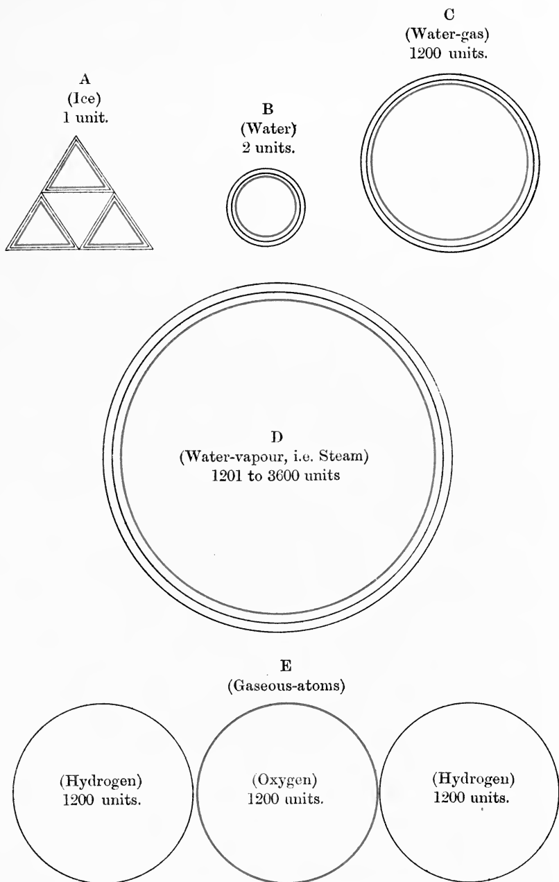
Fig. 5.—The figures represent in sections the various well marked but not rigid forms a water molecule assumes.
