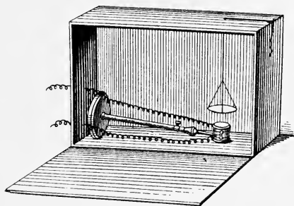
Fig. 6.—Thermopile with object acting upon it at a distance.
