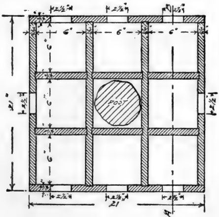
FLOOR PLAN Plans for a Martin house—Continued See also design on page 309
