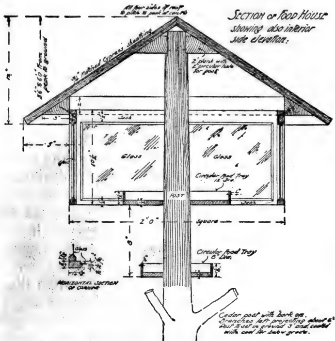
Plan for an "Audubon" food house.
