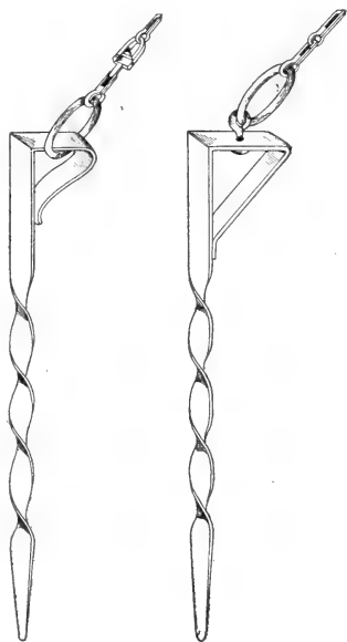
FIG. 5.—Iron stakes for wolf trap, with and without swivel.
