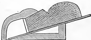
Fig. 8.—Bull-nose Plane in Section.
