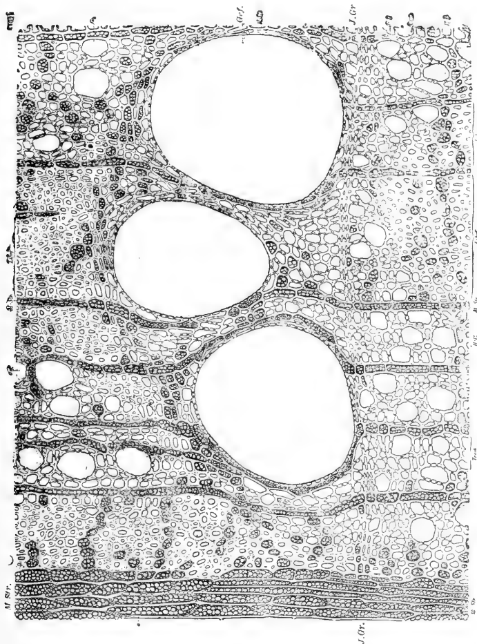
FIG. 27.—Transverse section of Oak, highly magnified. Cef. , Large tracheae; M. Str. , pith-rays, a large one to the left; L. Str. , wood-fibres; H. P. , wood-parenchyma; Trach. , tracheids; J. Cr. , boundary of annual ring. (After Kny, from The Oak , by permission of Prof. Marshall Ward and Messrs. Kegan Paul, Trench, Trübner & Co.)
