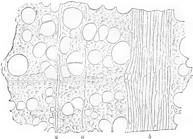
FIG. 26.—Transverse section of Beech ( Fagus sylvatica ). Magnified 100 times. a , narrow pith-ray; b , broad pith-ray; c , boundary of an annual ring. The large pores are transverse sections of vessels (tracheæ). The thick-walled elements with narrow lumina are wood-fibres; those with thinner walls and wider lumina, wood-parenchyma or tracheids. (From Hartig's Timbers and how to know them , by permission of Dr. Somerville and Mr. David Douglas.)
