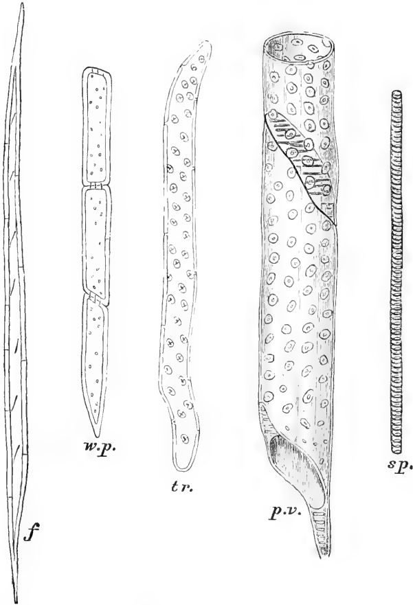
FIG. 10.—Elements of Oak Wood, highly magnified. f , fibre; w.p. , part of row of wood-parenchyma cells; tr. , tracheid; p.v. , trachea (part of); sp. , part of a spiral vessel. (From The Oak , by permission of Prof. Marshall Ward and Messrs. Kegan Paul, Trench, Trübner & Co.)
