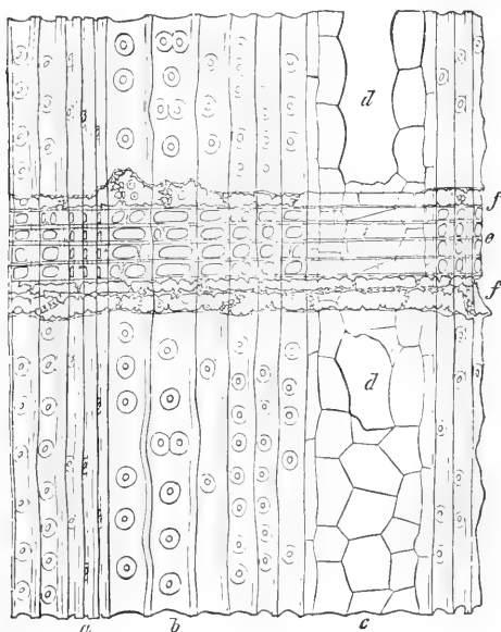
FIG. 30.—Radial section of Scots Fir ( Pinus sylvestris ). Magnified 100 times. a , narrow tracheids of autumn wood with small bordered pits on their radial walls; b , broad spring tracheids; cd , resin-duct lined with epithelium; e , parenchyma of pith-ray with large simple pits; f , tracheids of pith-ray with small bordered pits and dentate projections. (From Hartig's Timbers and how to know them , by permission of Dr. Somerville and Mr. David Douglas.)
