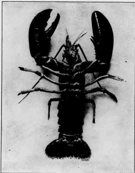
Female lobster with eggs.
