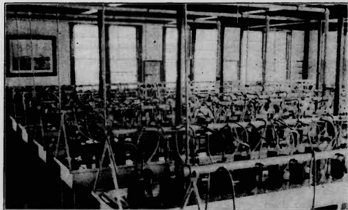
Interior of lobster-hatching plant showing jars in operation.
