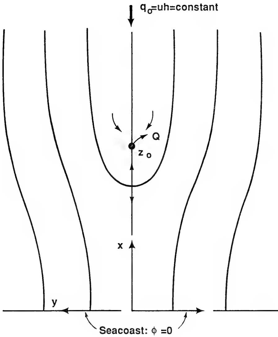
Fig. 8.7. Flow to a Single Well Along a Seacoast.
