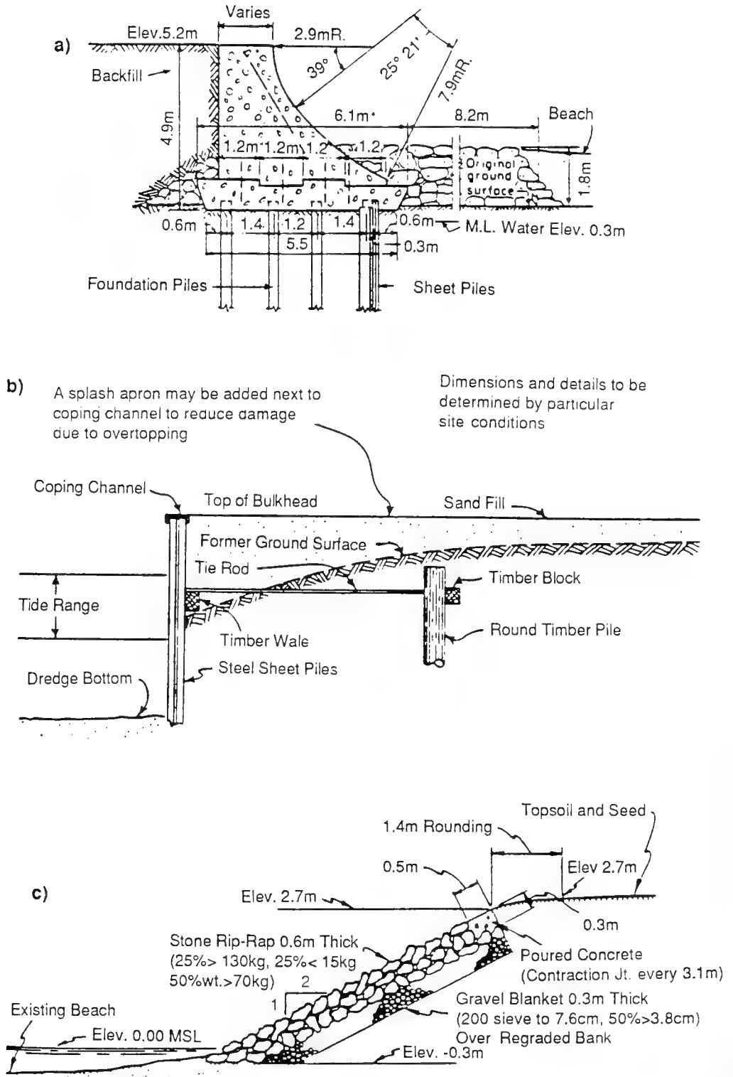
Fig. 6.7. Typical Cross sections of a) Seawall, b) Bulkhead and c) Revetment (adapted from Shore Protection Manual, U.S. Army Corps of Engineers, 1984).
