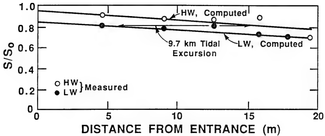
Fig. 9.4. High and Low Water Salinity Profiles through St. Marys Entrance, Florida and Cumberland Sound, Georgia (after Parchure, 1982).
