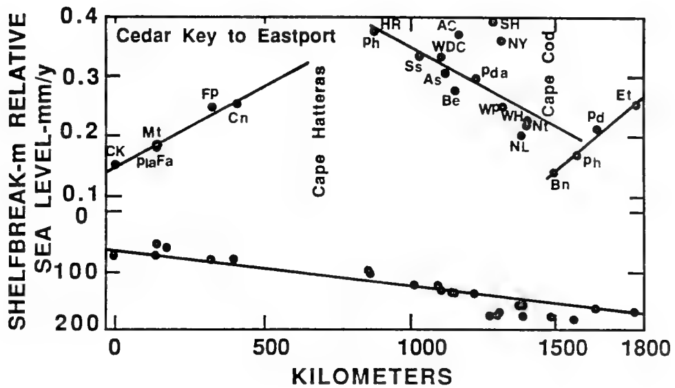
Fig. 2.2. Mean Annual Relative Sea Level Changes During 40-Year Record. Lines Define Three Main Segments of East Coast with Differing Sea Level Trends. Reprinted with permission from Continental Shelf Research, Volume 2, D. C. Aubrey and K. O. Emery, "Eigenanalysis of recent United States sea levels," copyright 1983, Pergamon Press plc.
