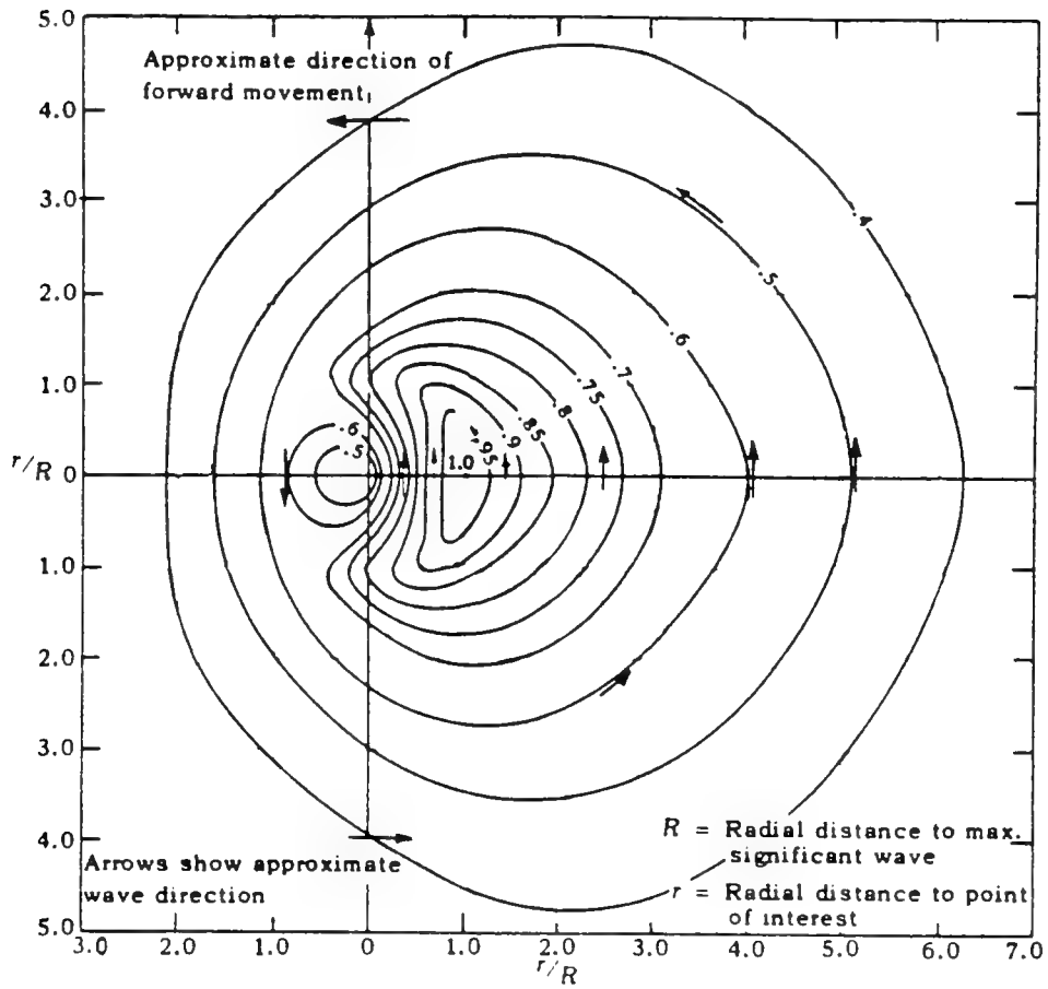
Fig. 5.2. Isolines of Non-Dimensional Significant Wave Height for Hurricane-generated Wind-waves (after Bretschneider, 1959).
