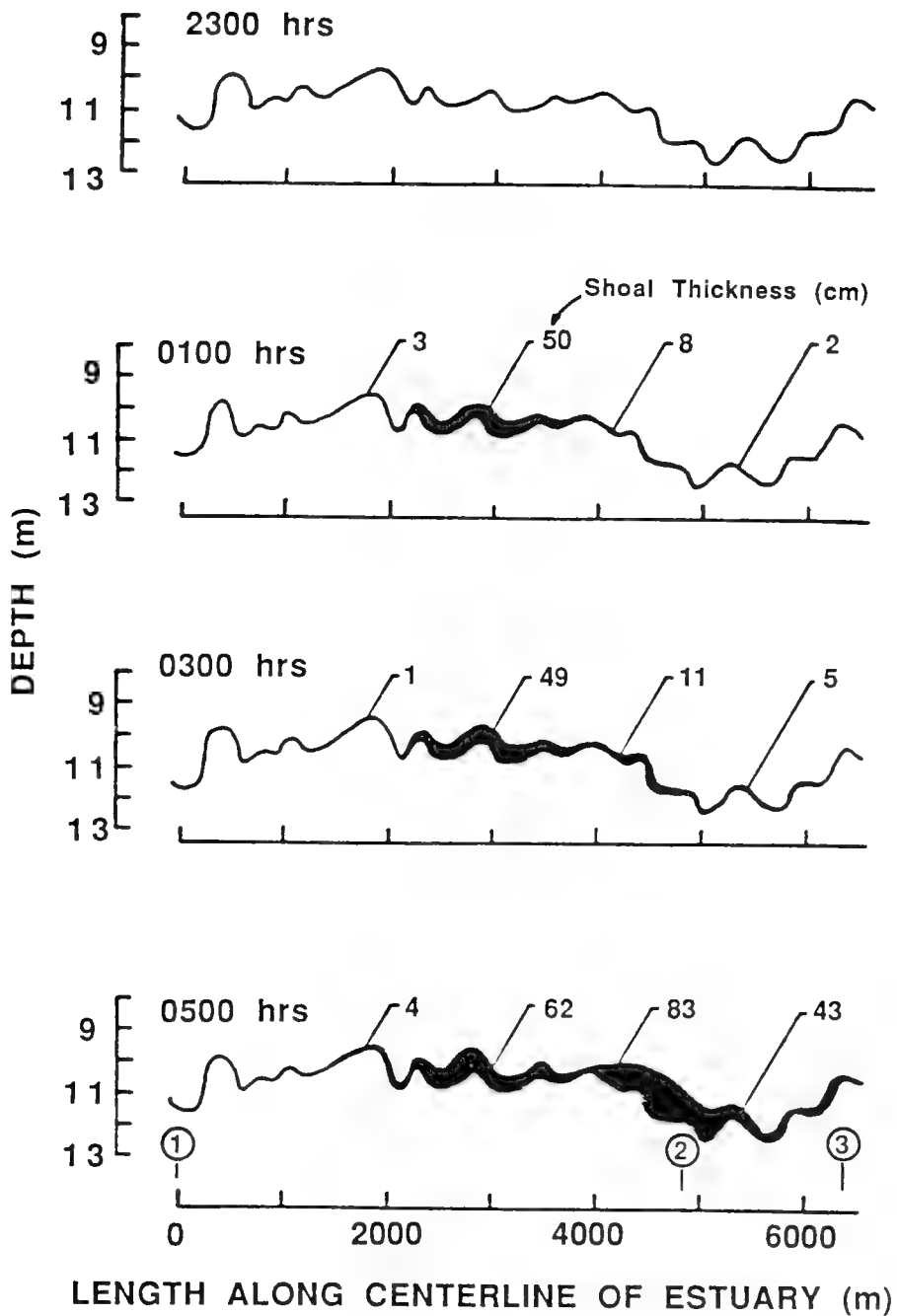
Fig. 10.4. Time History of Bottom Sediment Movement in Savannah Harbor Estuary, Georgia (after Ariathurai et al., 1977).
