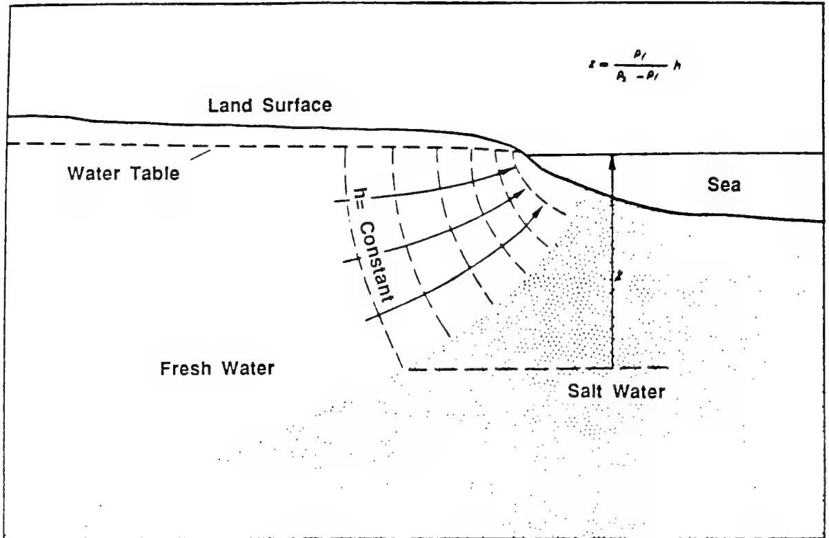
Fig. 8.2. Balance between Fresh Water and Salt Water in a Coastal Aquifer in which the Salt Water is Static (after Cooper, 1964).
