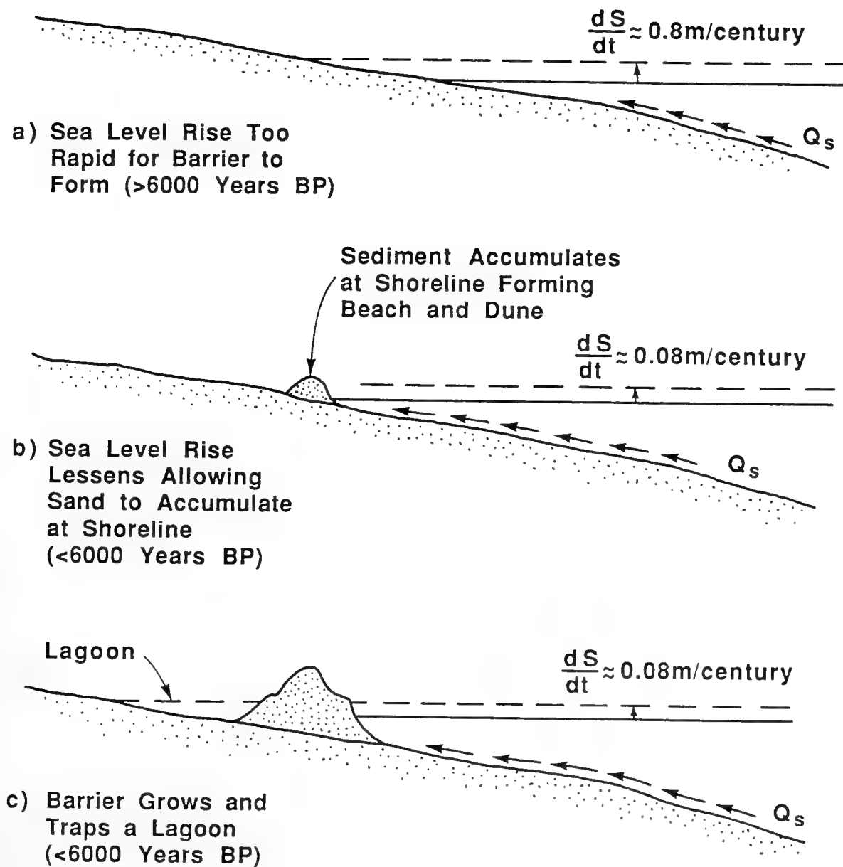
Fig. 7.6. The Role of Shoreward Sediment Transport, Q_s , Across the Shelf and Rate of Sea Level Rise in Causing Barrier Island Formation (from Dean, 1987, courtesy of Shore and Beach).
