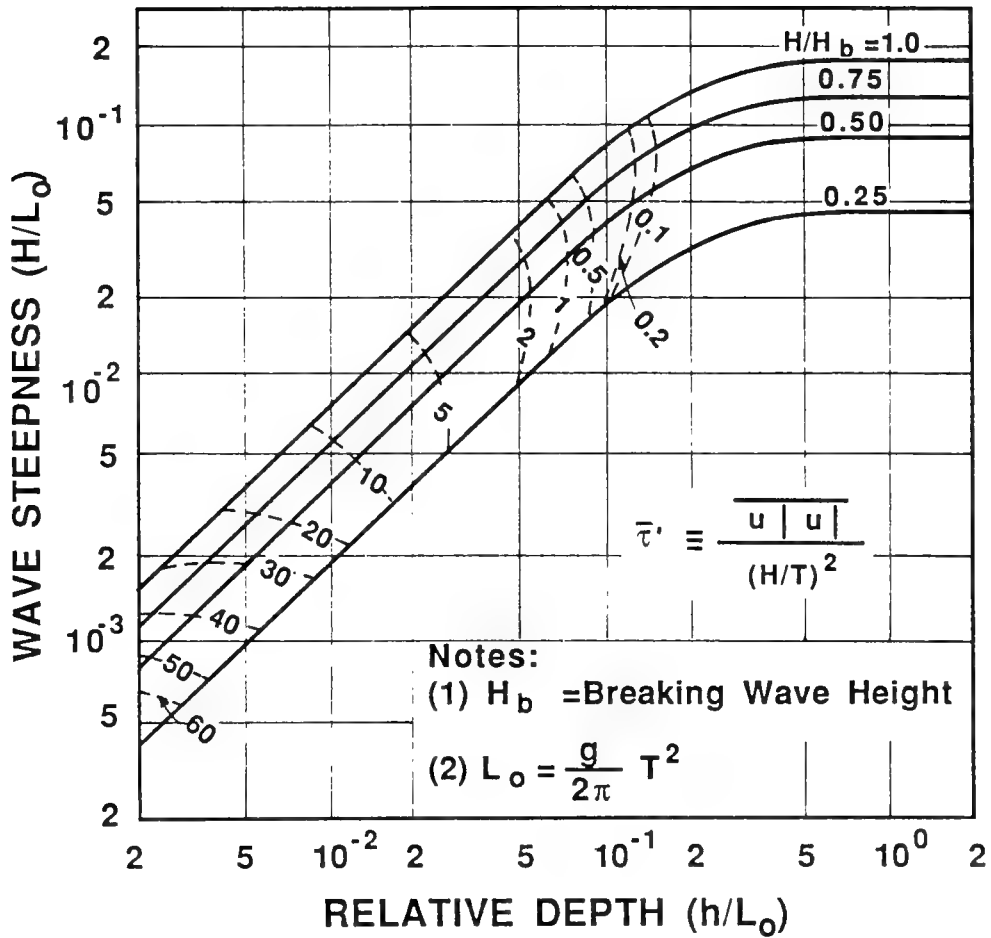
Fig. 7.11. Isolines of Non-dimensional Average Bottom Shear Stress \bar{\tau} vs Relative Depth h/L_0 , and Wave Steepness, H/L_0 (from Dean, 1987, courtesy of Shore and Beach).
