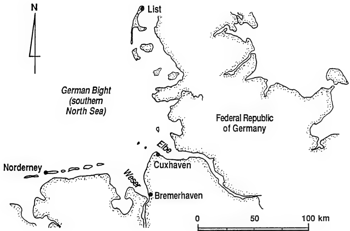
Fig. 4.2. Locations of Four Tide Gages in the German Bight.
