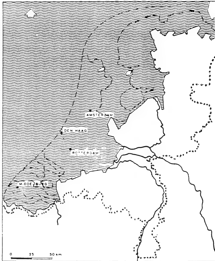
Fig. 6.6. Shoreline of Holland if There Were No Dikes, Showing a 50% Loss in Land Area (after Lingsma, 1966).
