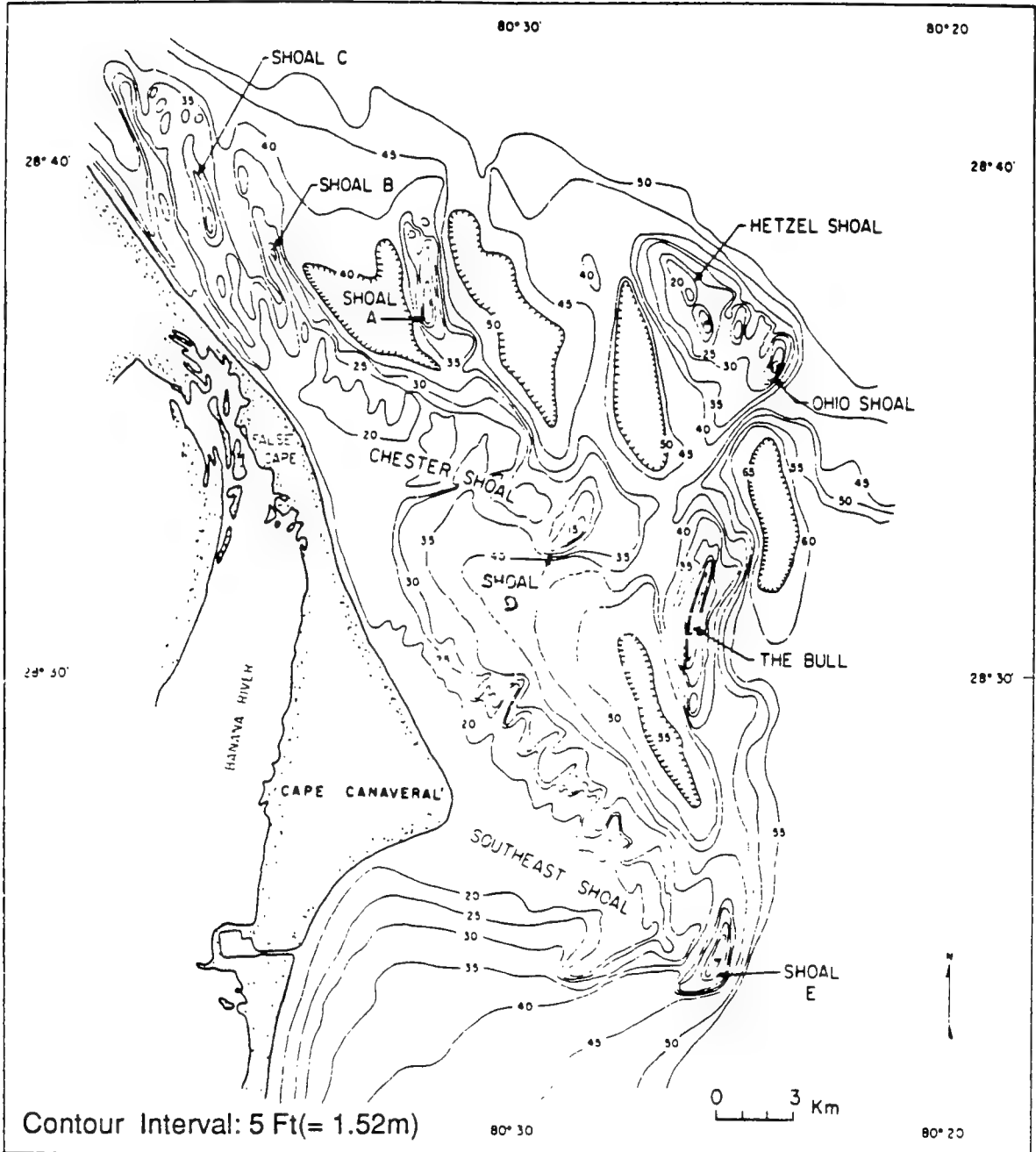
Fig. 6.2. The Shoal System at Cape Canaveral, Florida (after Field and Duane, 1974).
