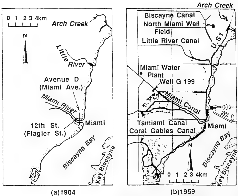
Fig. 8.9. Progressive Saltwater Intrusion in the Vicinity of Miami, FL, 1904 to 1959 (reprinted with permission from D. K. Todd, Groundwater Hydrology , copyright 1980, John Wiley & Sons, Inc.).
