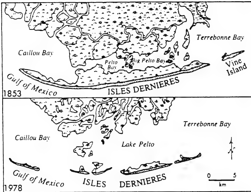
Fig. 6.1. Historical Shoreline Changes at the Isles Dernieres, Louisiana (after Penland et al., 1985).
