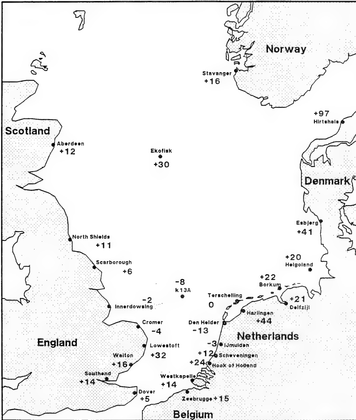
Fig. A.11. Percent Change in Tidal Amplitude, with a Sea Level Rise of 5 m.
