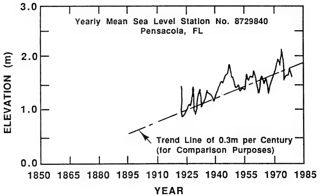
Fig. 2.6. Average Annual Sea Level Variations for Pensacola, Florida (adapted from Hicks et al., 1983).
