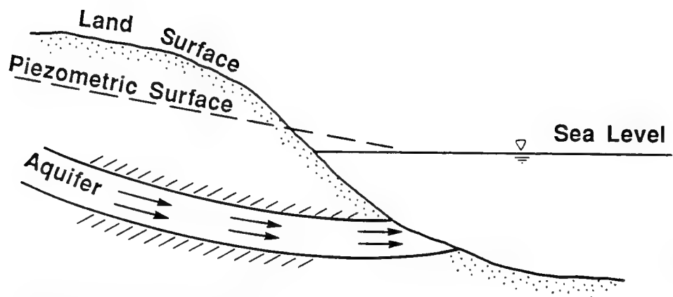
b) Confined Aquifer
