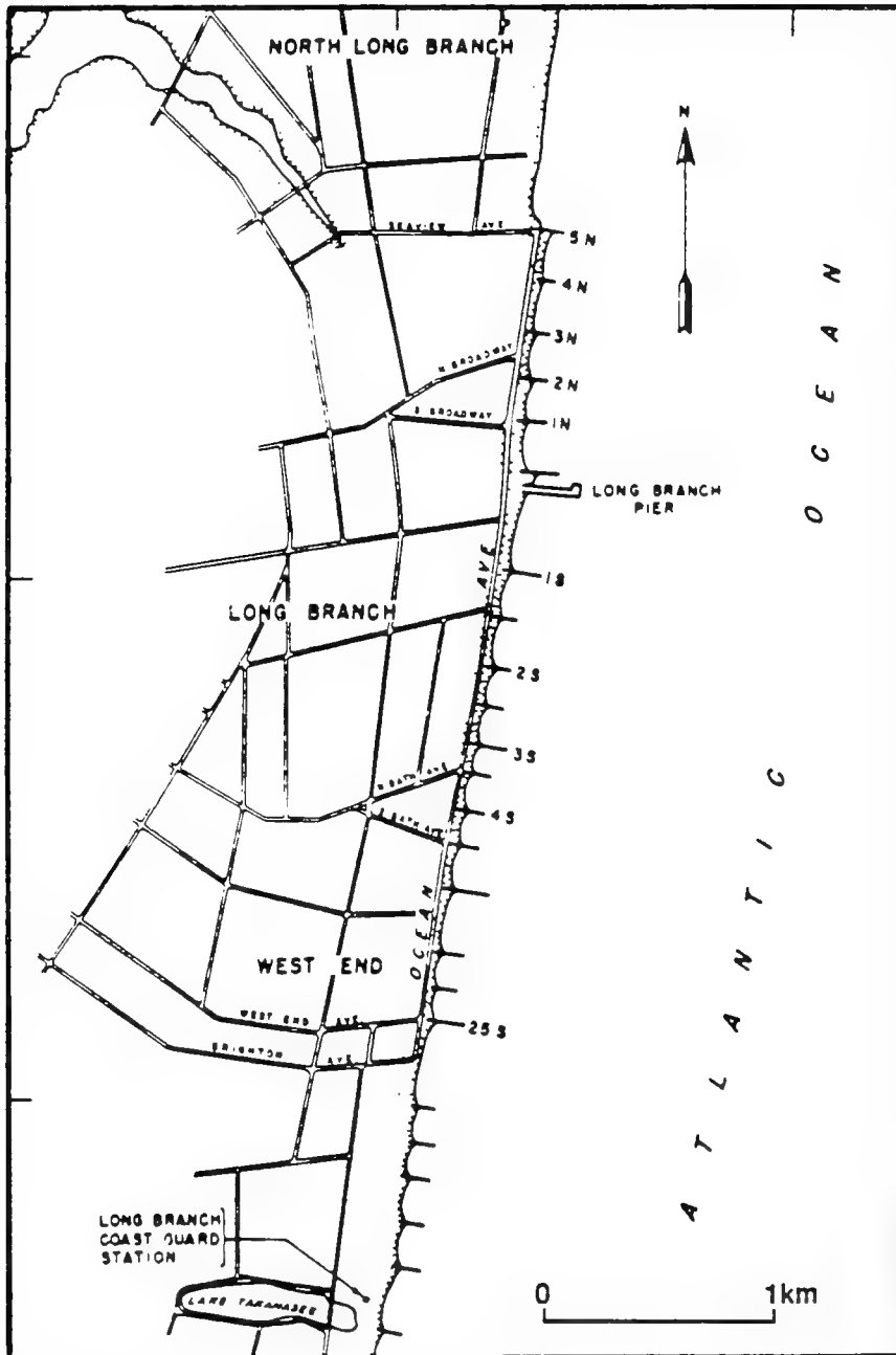
Fig. 6.10. Groin Field at Long Branch, New Jersey (after Army Corps of Engineers, 1964).
