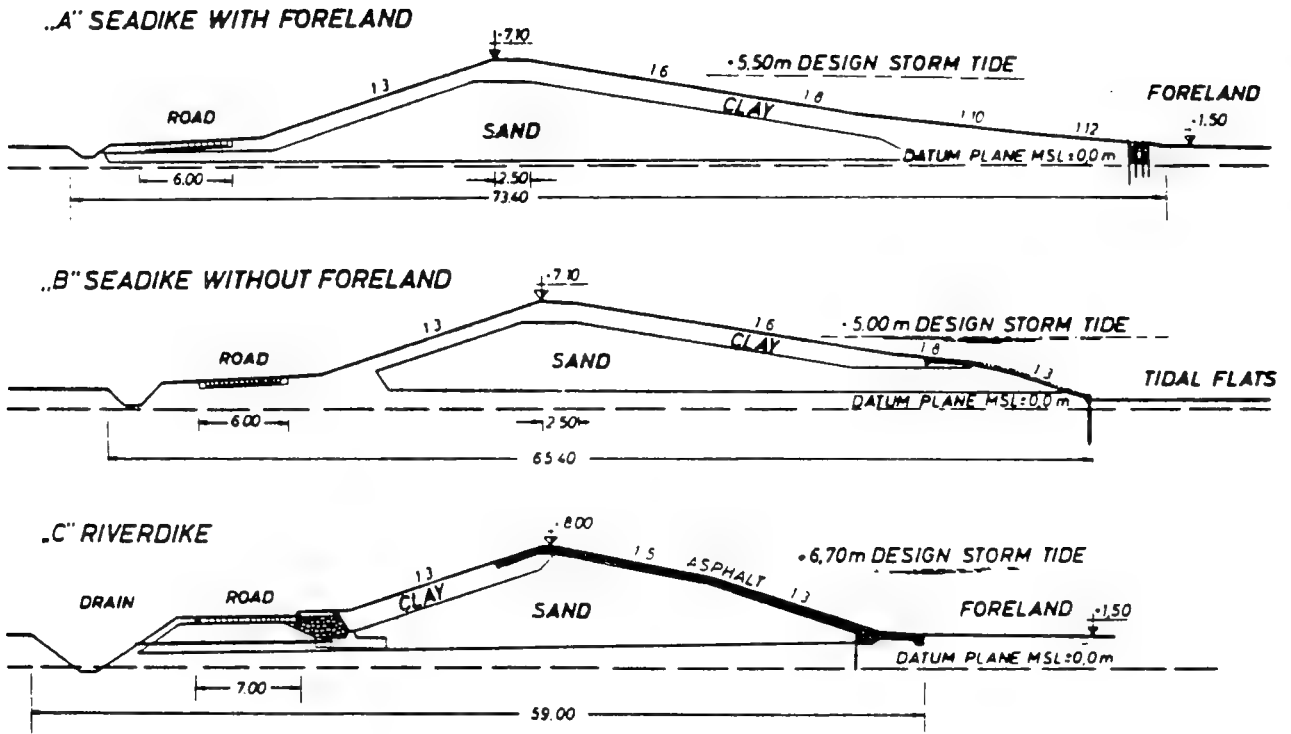
Fig. 6.5. Examples of Design Cross-sections for Sea Dikes (after Kramer, 1971).
