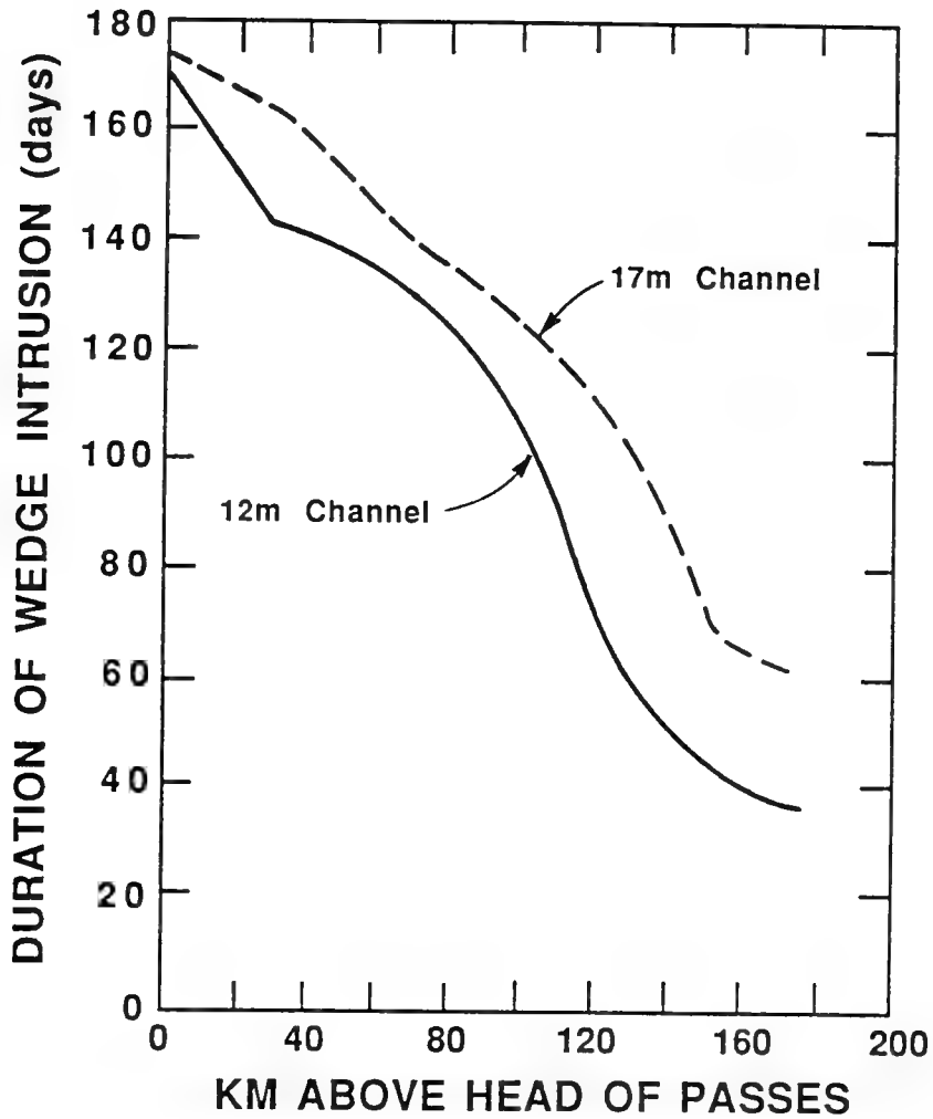
Fig. 9.5. Effect of Channel Deepening on the Duration of Wedge Intrusion in the Lower Mississippi River (after Johnson et al., 1987).
