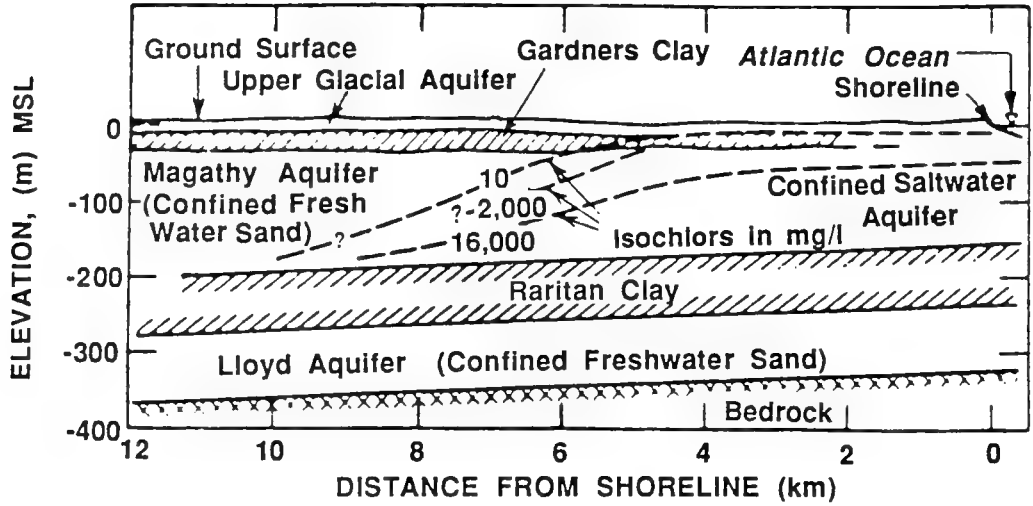
Fig. 8.8 Profile through Aquifer at Far Rockaway, Nassau County, Long Island, Showing Location of Salinity Front as a Result of Pumping (reprinted with permission from D. K. Todd, Groundwater Hydrology , copyright 1980, John Wiley & Sons, Inc.).
