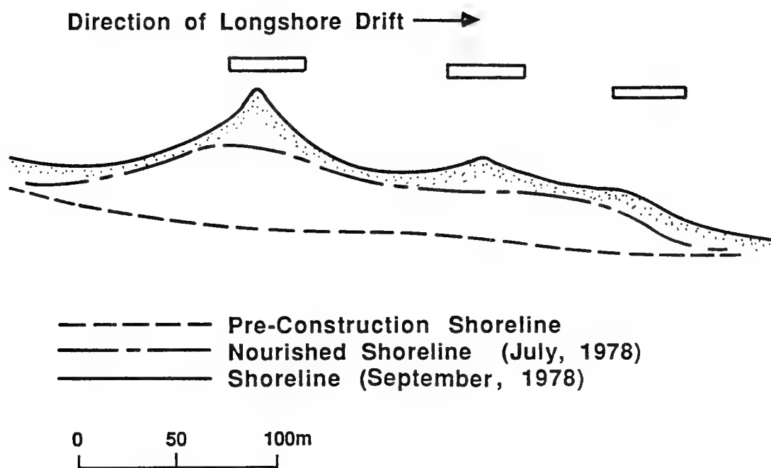
Fig. 6.9. Breakwater Project and Shoreline Response at Presque Isle, Pennsylvania.
