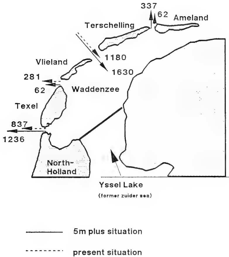
Fig. A.12. The Change in the Residual Transports in the Wadden Sea, with a Sea Level Rise of 5 m.
