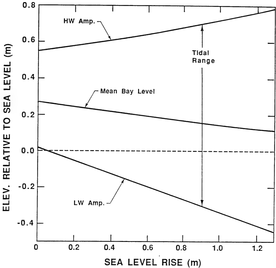
Fig. 4.3. Response of a Shallow Inlet/Deep Bay System to Sea Level Rise: Changes in Mean Bay Level and Tidal Amplitudes (based on computations by Mann, 1987).
