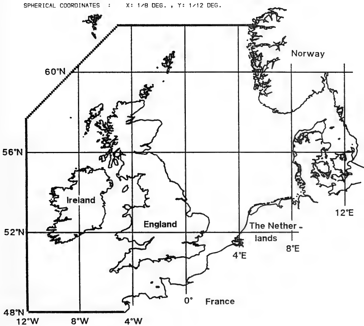
Fig. A.9. The Outlines of the Continental Shelf Model.
