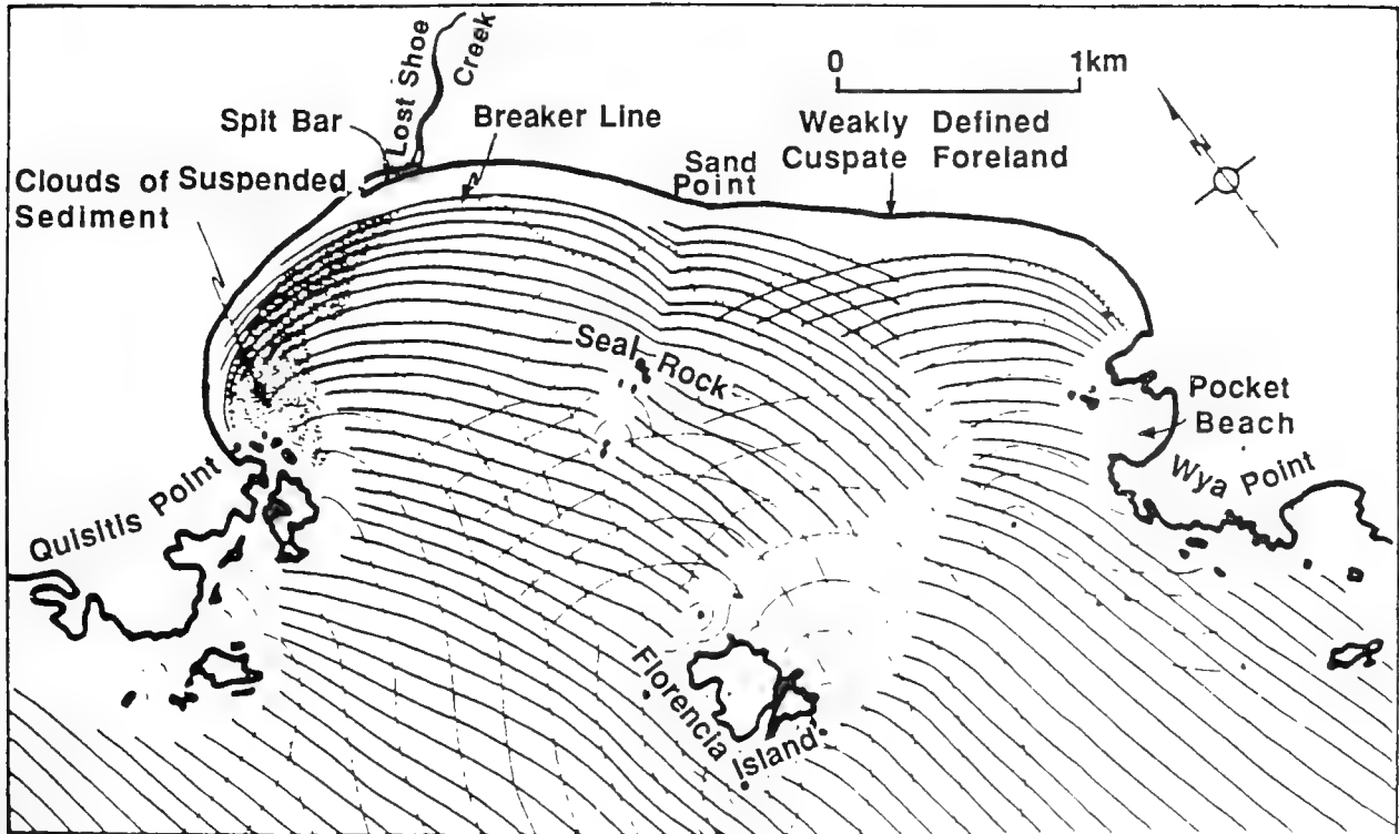
Fig. 6.4. Shoreline Between Two Headlands at Wreck Bay, Vancouver Island, with Observed Wave Patterns (from Bremmer and LeBlond, 1974, with permission from the Society of Economic Paleontologists and Mineralogists).
