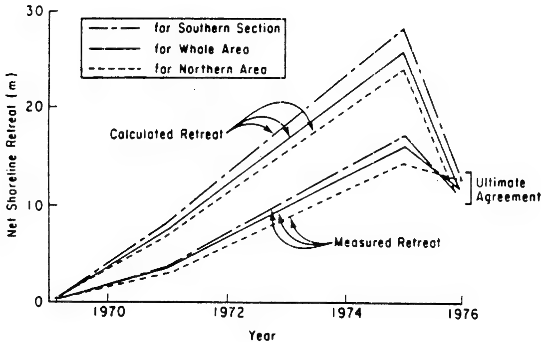
Fig. 7.4. Comparison of Predicted and Measured Shoreline Changes Due to Water Level Increases, Eastern Shore of Lake Michigan (after Hands, 1983). Reprinted with permission from Handbook of Coastal Processes and Erosion. Copyright CRC Press, Inc., Boca Raton, Florida.
