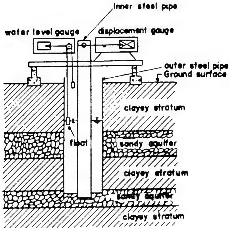
Fig. 3.2. Device for Monitoring Compaction and Groundwater Elevation (after Murayama, 1970).
