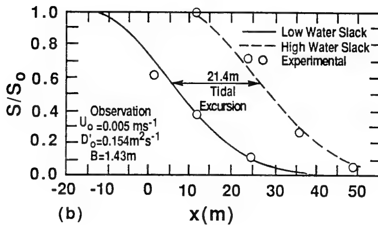
Fig. 9.2. Longitudinal Salinity Distribution in a Model Tidal Channel: a) Test No. 2, b) Test No. 16 (after Harleman and Abraham, 1966).
