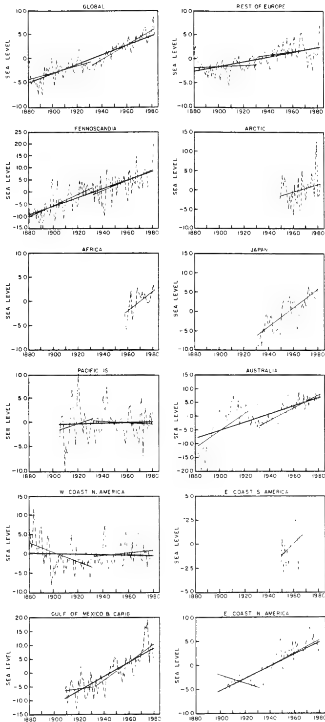
Fig. A.1. Global and Regional Sea Level Curves, 1880-1980. Heavy line represents least-squares slope for the past century. Lighter lines represent slopes for the intervals 1880-1931 and 1932-1980. Units are in centimeters (from Gornitz and Lebedeff, 1987).
