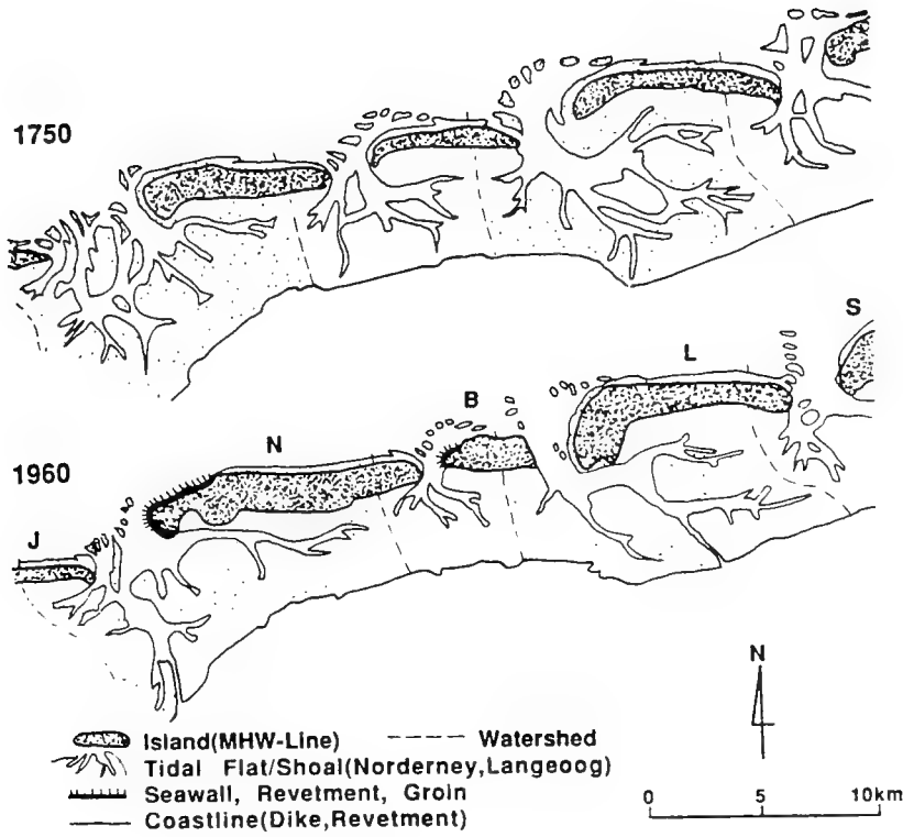
Fig. 10.1. East Frisian Islands in 1750 and in 1960 (after Kunz, 1987).
