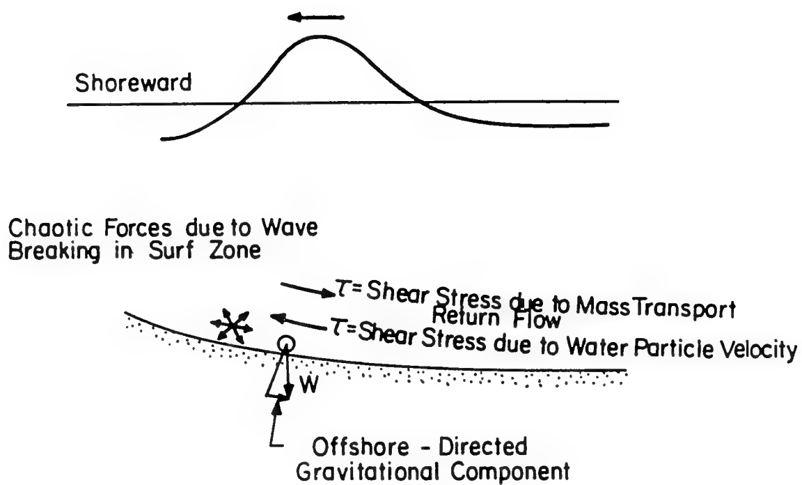
Fig. 7.10. Dominant Forces Acting on a Sediment Particle Resting on the Bottom.
