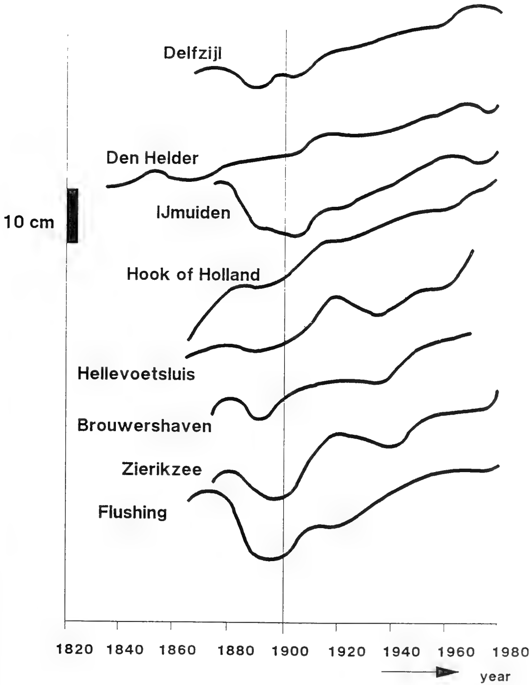
Fig. A.3. Filtered Mean Sea Levels of the Main Dutch Gages.
