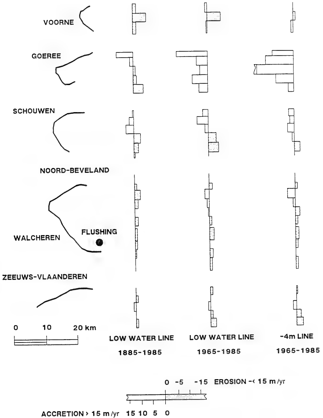
Fig. A.7. Erosion and Accretion of the Delta Islands.
