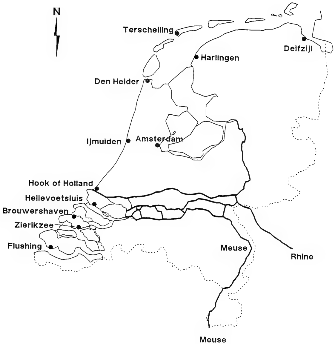
Fig. A.4. Map Showing the Main Dutch Gages.
