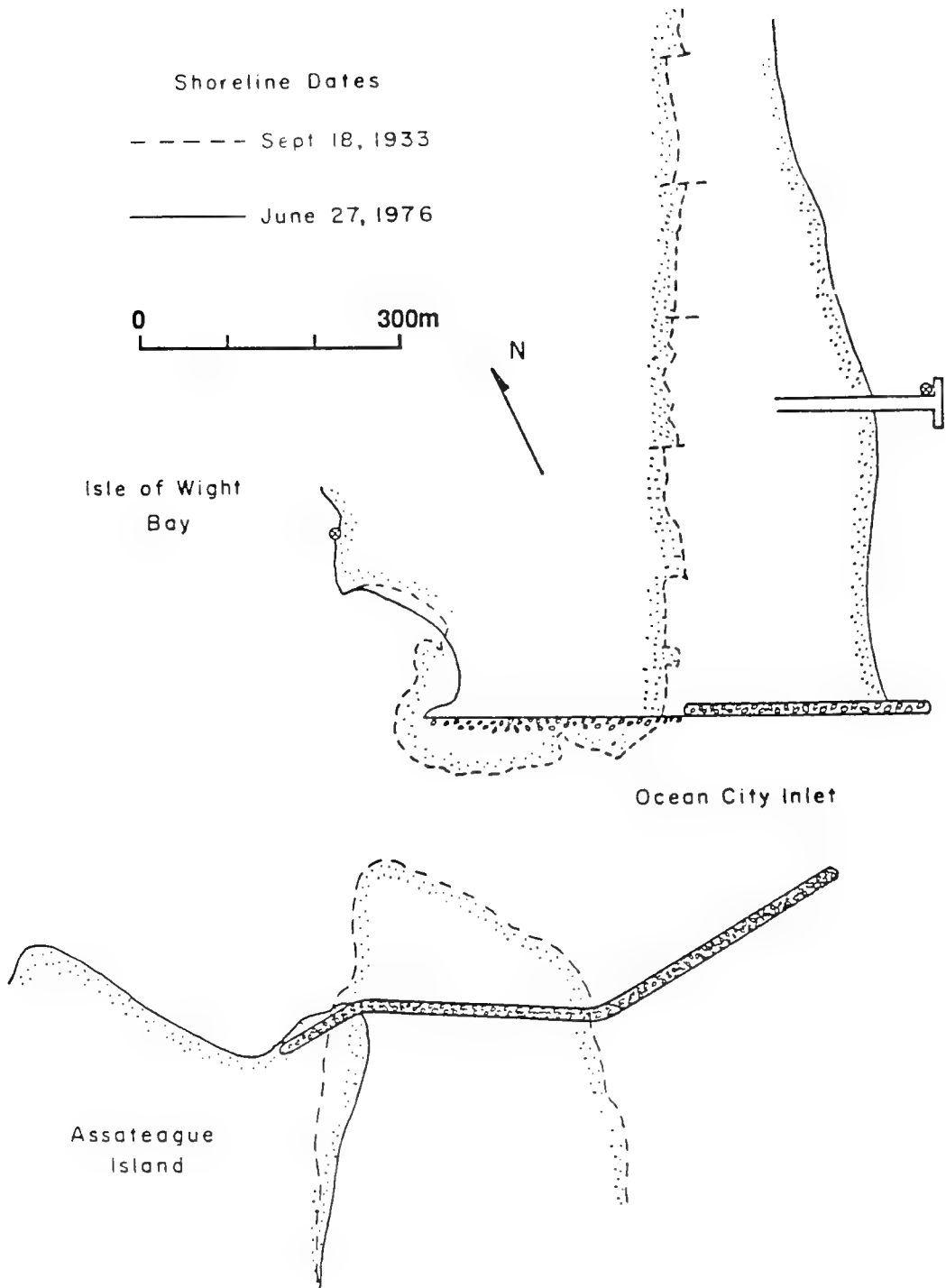
Fig. 6.11. Shoreline Response to Jetty Construction at Ocean City, Maryland (after Dean et al., 1979).
