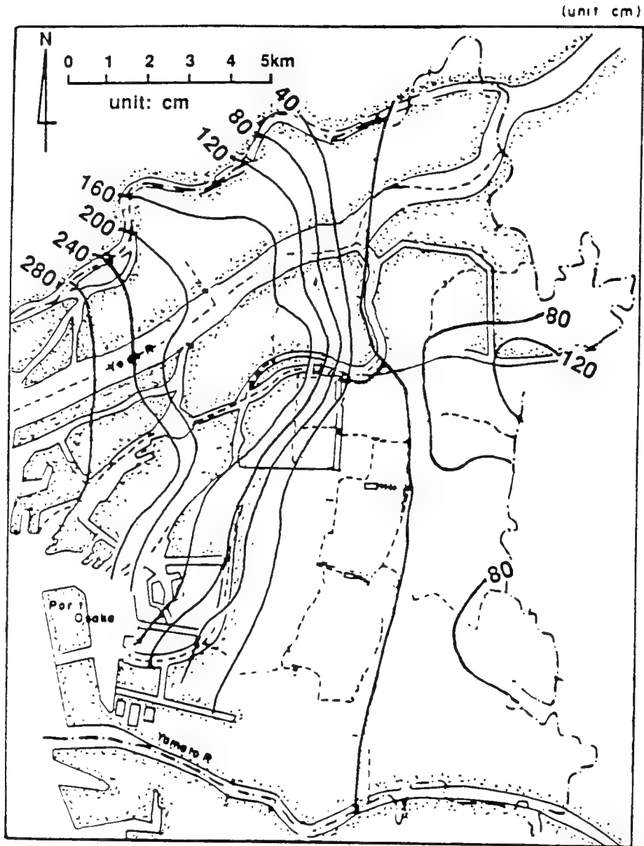
Fig. 3.3. Isolines of Total Subsidence (in cm) from 1935-1968 in Osaka, Japan (after Murayama, 1970).
