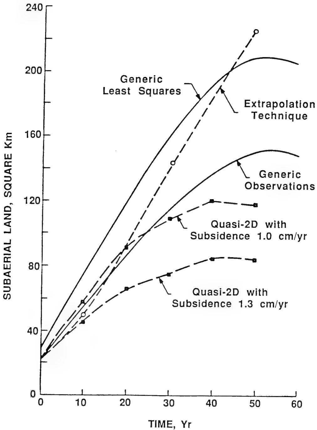
Fig. 10.3. Time Rate of Subaerial Land Growth in Atchafalaya Bay, Louisiana, Calculated by Different Approaches (after McAnally et al., 1984).
