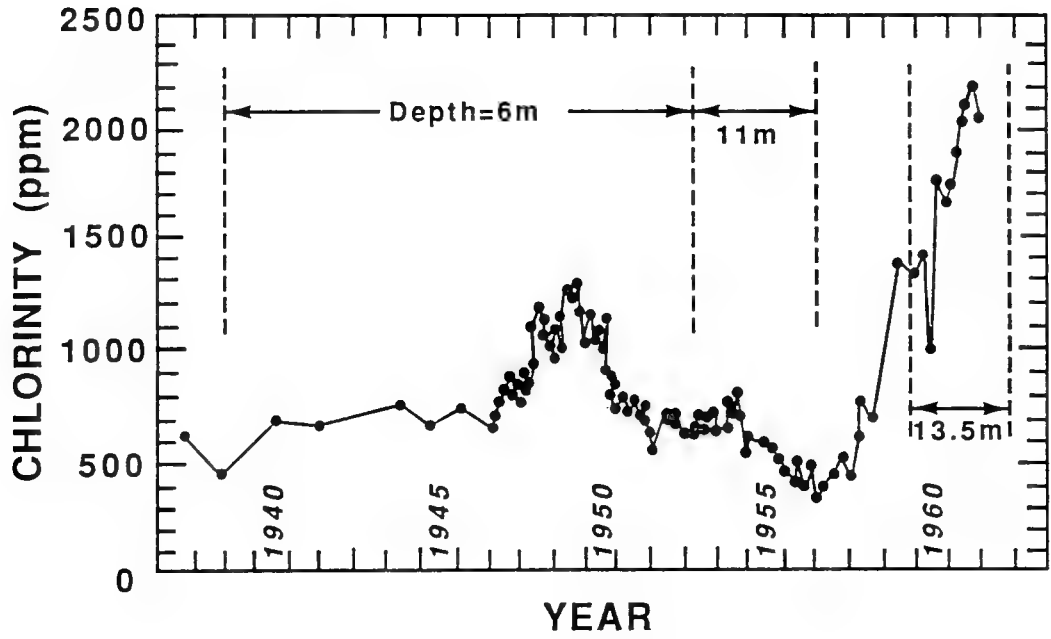
Fig. 9.3. Salinity (Chlorinity) Variation with Years in Lake Maracaibo (after Partheniades, 1966).
