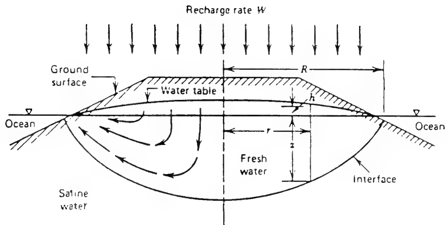
Fig. 8.6. Freshwater Lens Under a Circular Oceanic Island Under Natural Conditions (reprinted with permission from D. K. Todd, Groundwater Hydrology , copyright 1980, John Wiley & Sons, Inc.).
