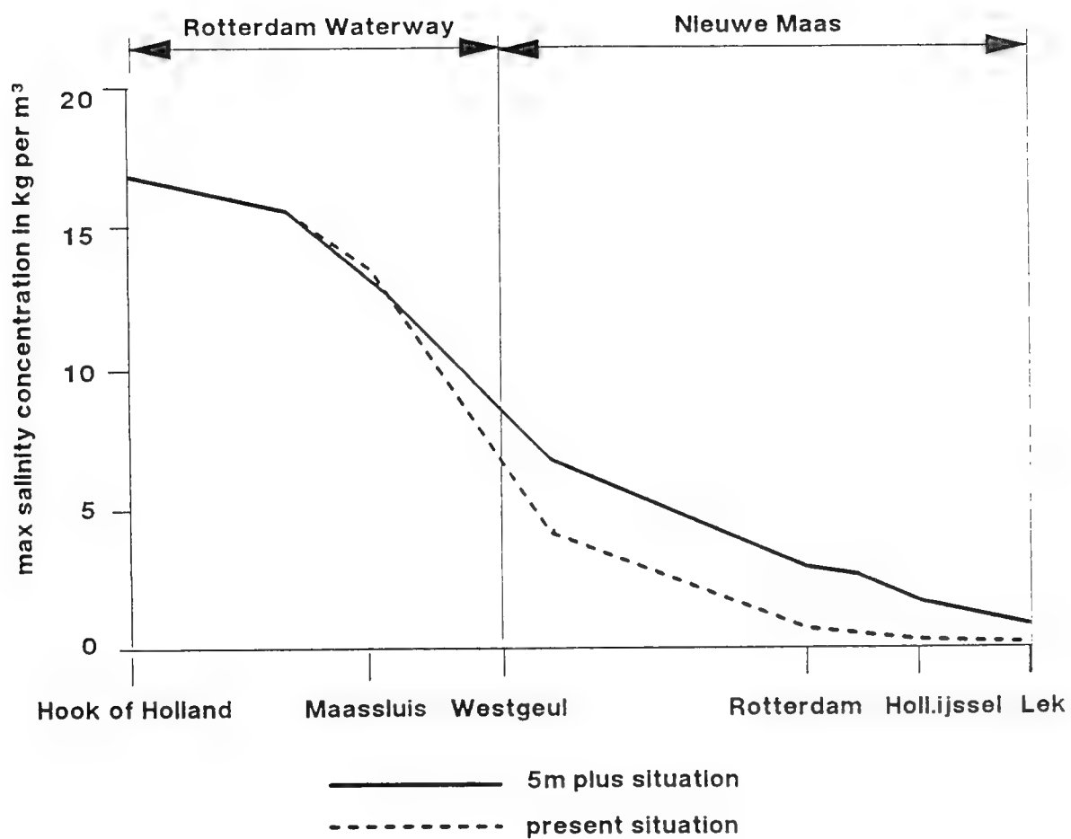
Fig. A.14. The Change in the Maximum Salinity Concentration during a Tidal Cycle in the Rhine Estuary, with a Sea Level Rise of 5 m.
