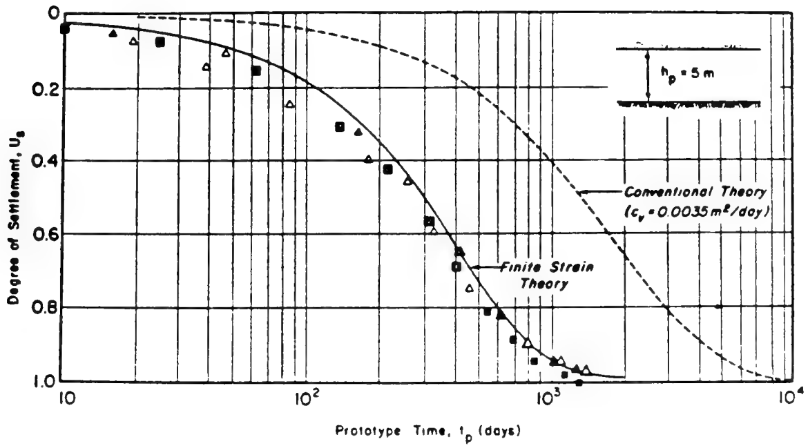
Fig. 3.1. Results of Centrifuge-aided Compaction in Comparison to Two Theories (after Schiffman et al., 1985).
