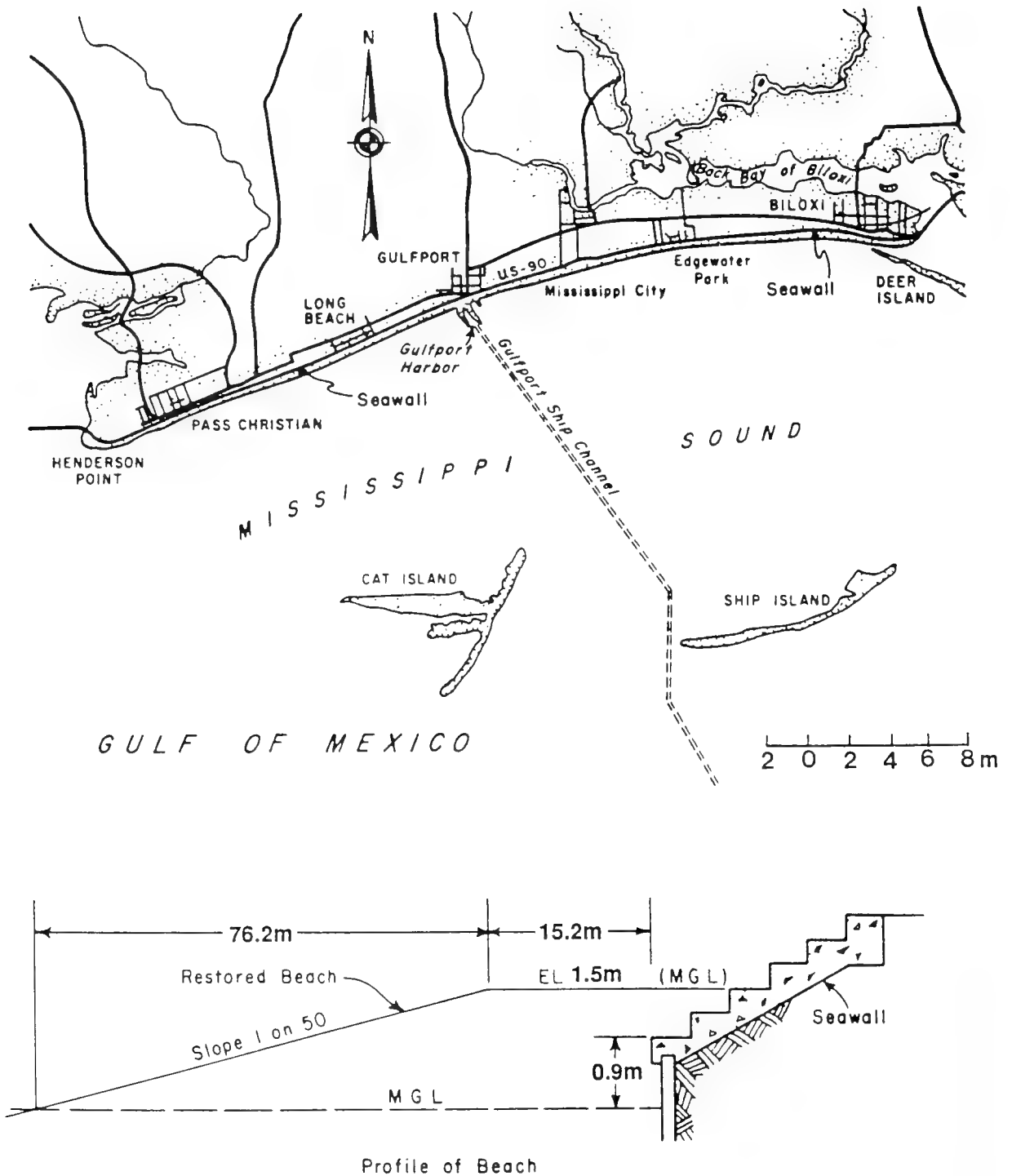
Fig. 6.12. Beach Nourishment Project at Harrison County, Mississippi (after Army Corps of Engineers, 1984).
