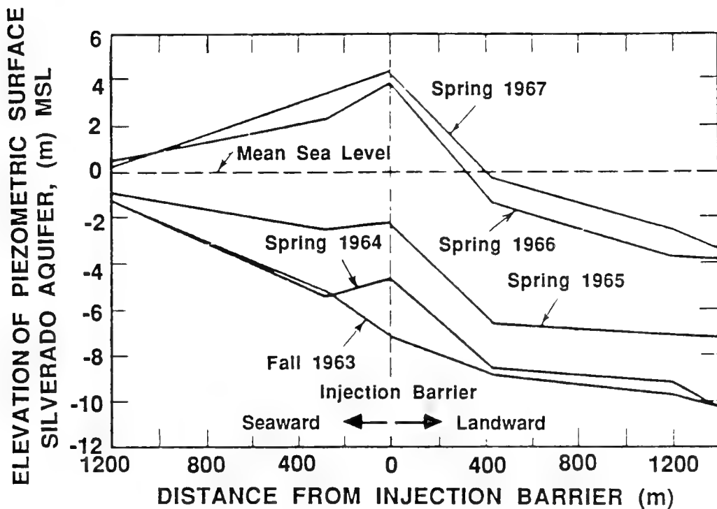
Fig. 8.10. Piezometric Pressure Profiles Perpendicular to the Seawater Intrusion Barrier in Los Angeles County for Various Times after Commencement of Injection in the Fall of 1963 (reprinted with permission from D. K. Todd, Groundwater Hydrology , copyright 1980, John Wiley & Sons, Inc.).
