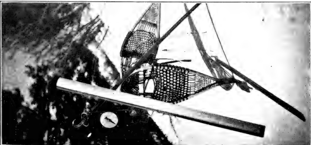
FIG. 1.—APPARATUS USED IN SNOW SUR- VEY—DENSITY TUBE, ALPENSTOCK, SNOWSHOES, AND SCALES.
