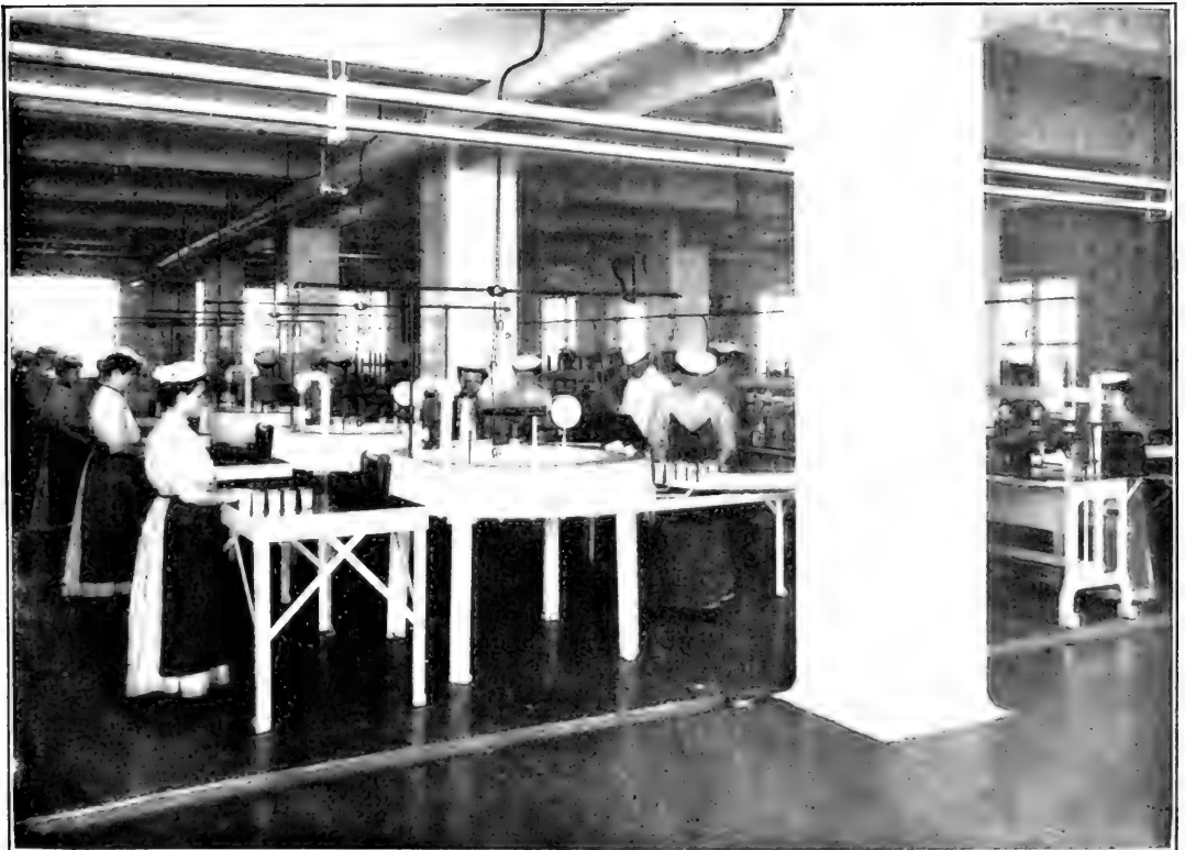
FIG. 2.—SEALING CANS IN VACUUM.
