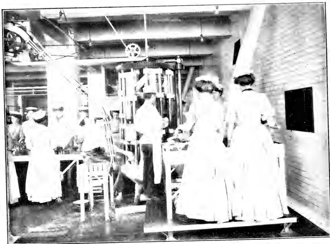
FIG. 2.—FILLING CANS WITH CORNED BEEF BY MACHINERY.
