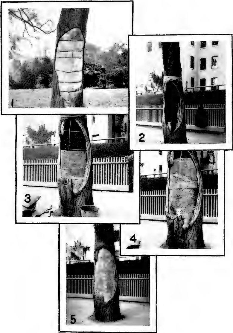
Fig. 1.—A large cavity in an elm filled with cement blocks separated by layers of tarred paper. Fig. 2.—An excavated cavity ready for treating and filling. Fig. 3.—The cavity shown in fig. 2, which has been nailed and partly filled with cement. The ends of the rods for reinforcing the concrete are sprung into shallow holes in the wood. The wire dam is sometimes allowed to remain embedded in the cement, though it is usually removed as soon as the cement has partially set. Fig. 4.—A later stage of the work shown in fig. 3. The height of the wire dam has been increased. Fig. 5.—The same cavity shown in figs. 2, 3, and 4, several days after the filling was completed.
