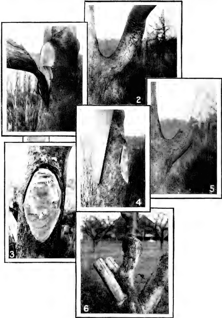
Fig. 1.—A heavy limb improperly cut, showing the stripping as the limb falls. (Compare with Figs. 2, 5, and 4.) Fig. 2.—Removing a heavy limb; the first cut on the underside is to prevent stripping. Fig. 3.—Removing a heavy limb; the oval scar has been somewhat pointed with a gouge above and below to facilitate healing. Fig. 4.—Removing a heavy limb; the third cut to remove the stub shown in fig. 5 has been completed. Fig. 5.—Removing a heavy limb; the second cut completed; the limb has fallen without any stripping. Fig. 6.—Improperly cut and untreated stubs. The bark of these stubs died mainly as a result of severing all the food-producing organs (leaves) above; decay has entered the trunk from these stubs. (Note that the successive stages in removing a heavy limb are shown in figs. 2, 5, 4, and 3, in the order indicated.)
