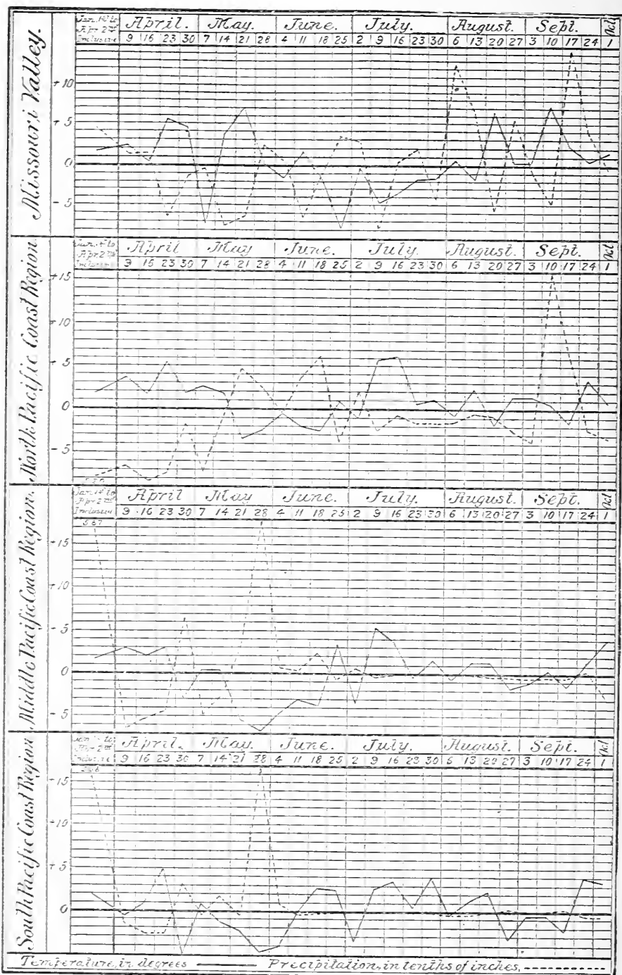
FIG. 17.—Temperature (degrees Fahrenheit) and precipitation (inches) departures for the season of 1906 from the normal of many years for the Missouri Valley and the Pacific coast.
