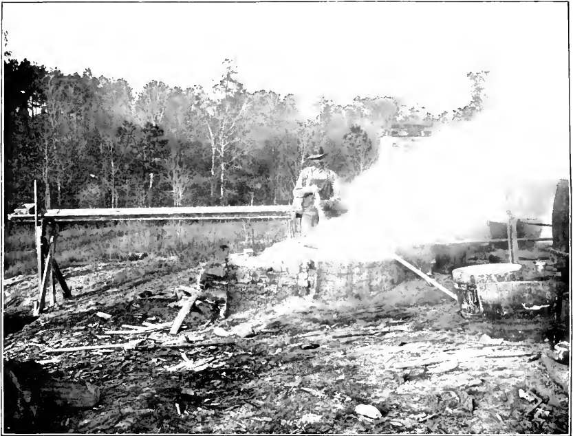
FIG. 1.—A SINGLE KETTLE FURNACE.
