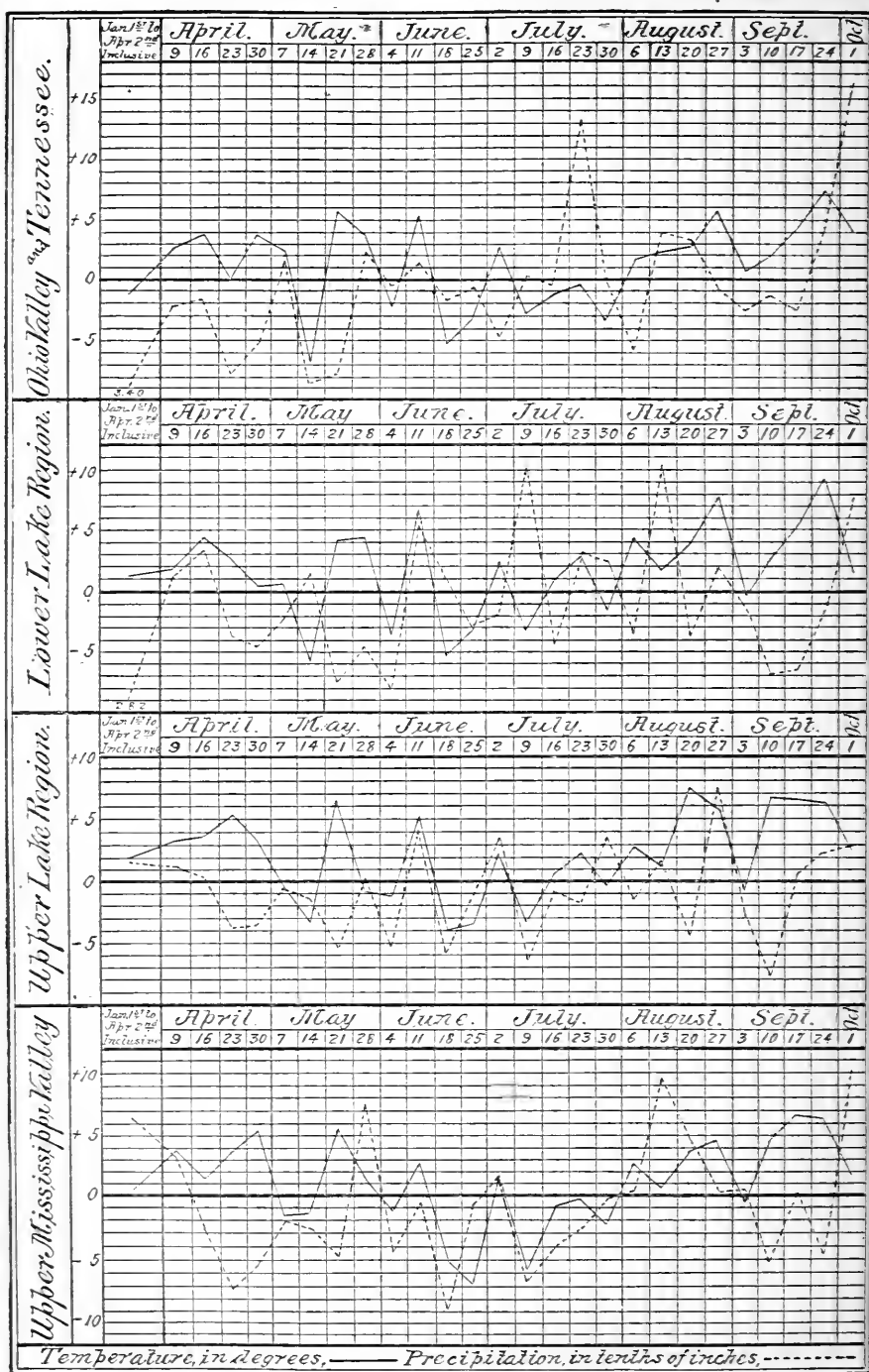
FIG. 19.—Temperature (degrees Fahrenheit) and precipitation (inches) departures for the season of 1906 from the normal of many years for the Lake region, the upper Mississippi Valley, the Ohio Valley, and Tennessee.
