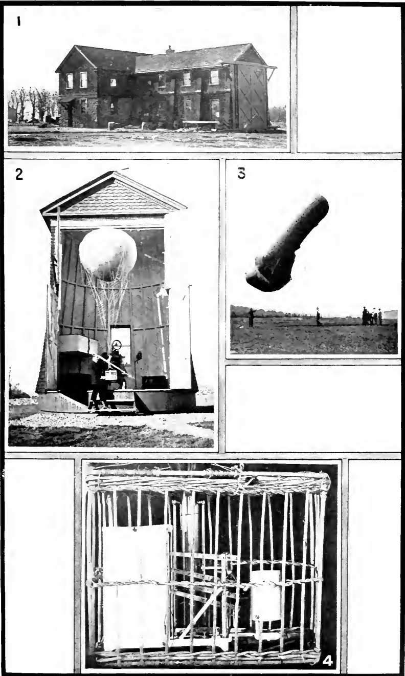
[1.—Power house and balloon shed. 2.—Revolving kite and balloon shed. 3.—The Siegfeld kite balloon. 4.—Hergesell balloon meteorograph in protecting basket.]
