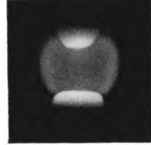
9. (Banden 2. Typus)
