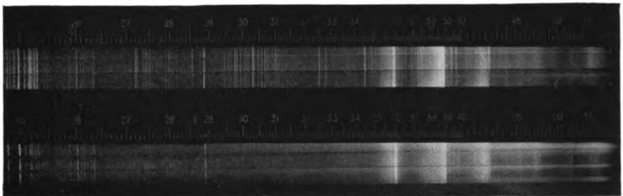
7. (Aluminium)
