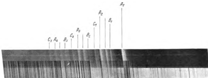
c) Benzonitril.
