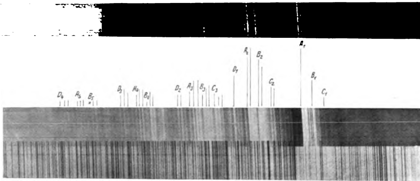
a) Fluorbenzol.
