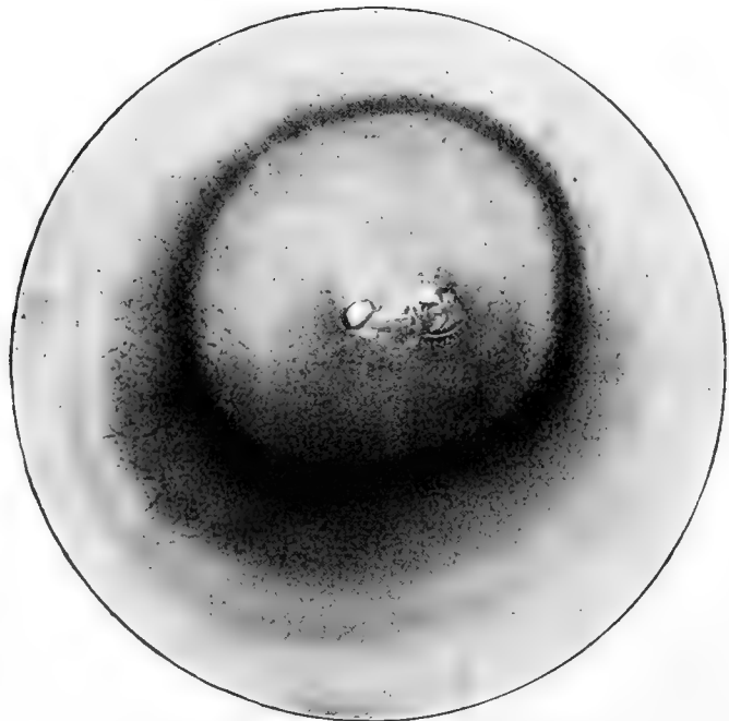
Fig. 2. Oscillatoria formosa .
