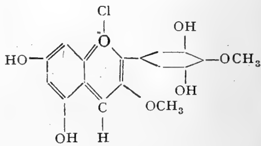
Oenidinchlorid.
