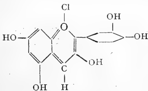
Cyanidinchlorid.
