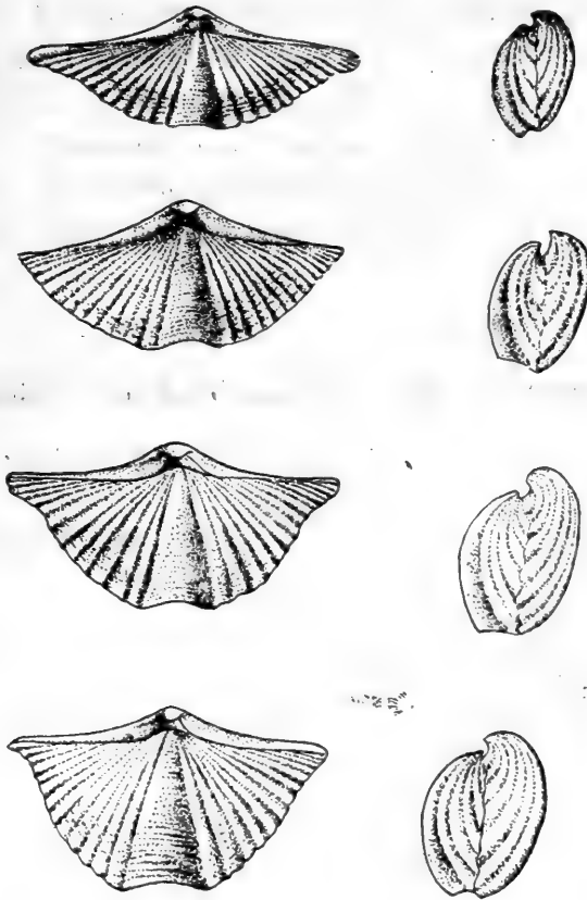
插图 9 示 Otospirifer shipaiensis Hou et Xian 的壳形变异 (Showing variations of the shell forms of Otospirifer shipaiensis Hou et Xian)
