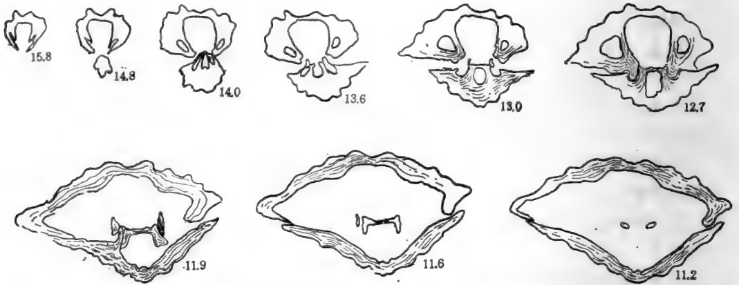
插图 6 Athyrisina wangi (sp. nov.) 连续横切面图 [Transverse serial sections of Athyrisina wangi (sp. nov.)], ×3.7
