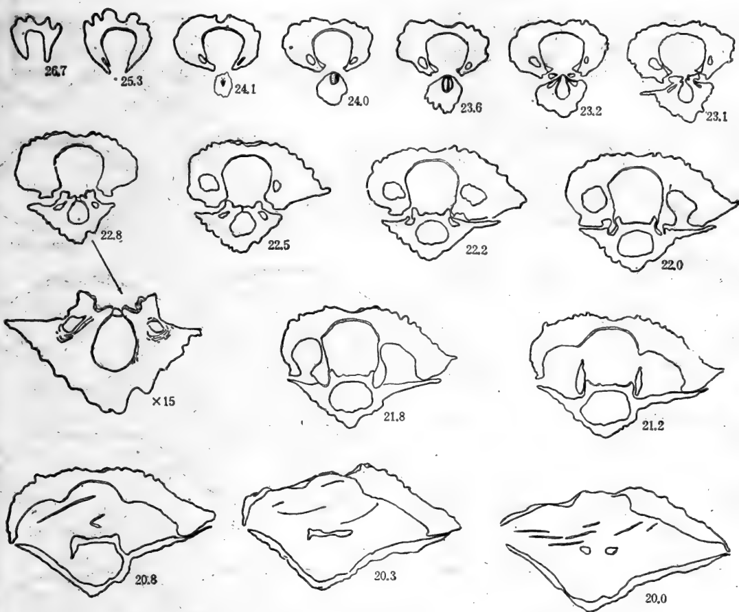
插图4 Kwangsia yohi Grabau 连续横切面图 (Transverse serial sections of Kwangsia yohi Grabau), \times 2
