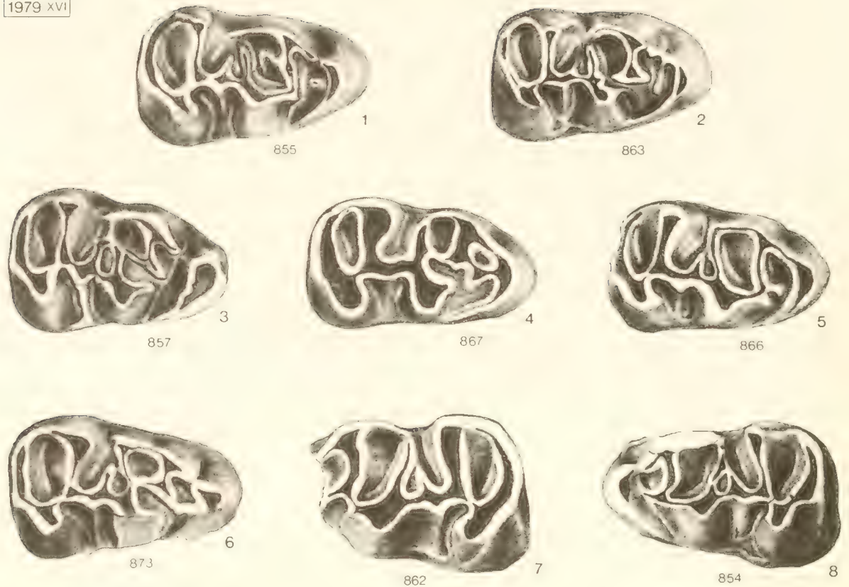
Abb. 12: Eumyarion cf. weinfurteri (SCHAUB & ZAPFE) aus Puttenhausen. re. M_1 (1–6), li. M_1 (7–8). \times 25
