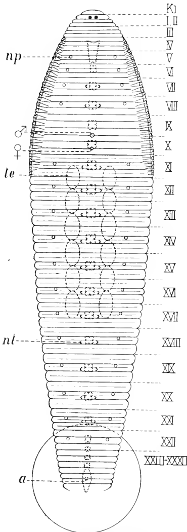
Fig. 2. Clepsine fimbriata .
